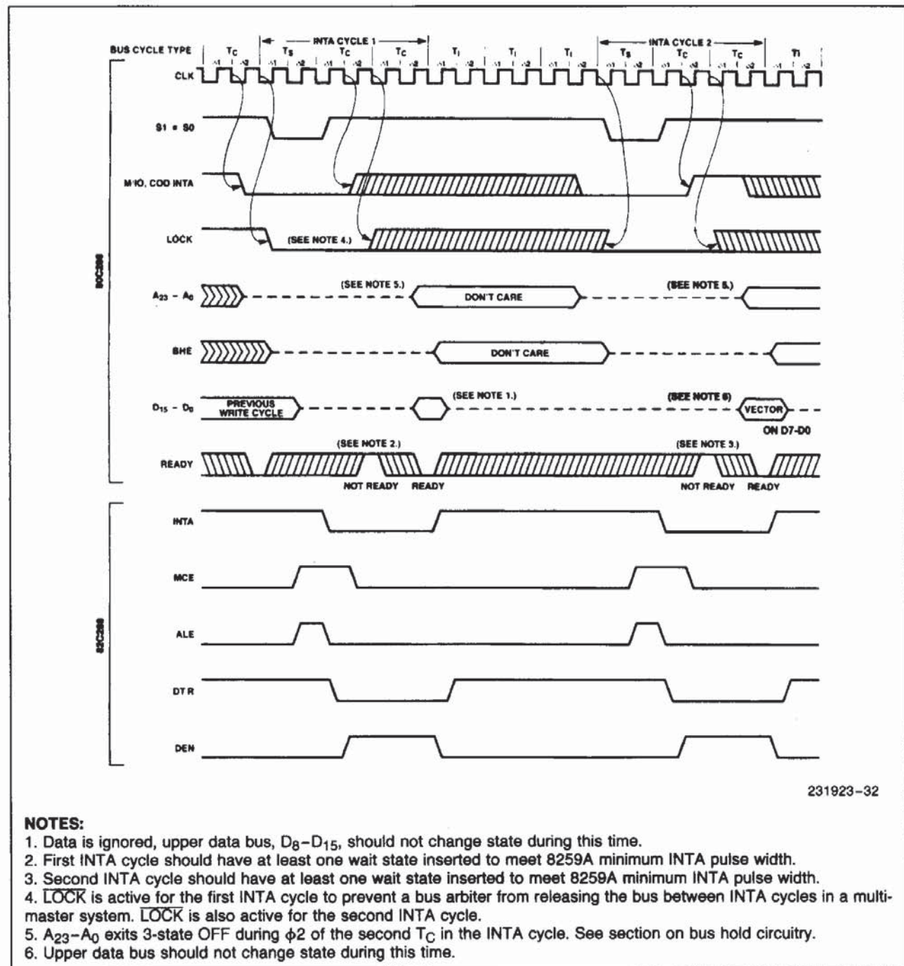
Figure 30. Interrupt Acknowledge Sequence
