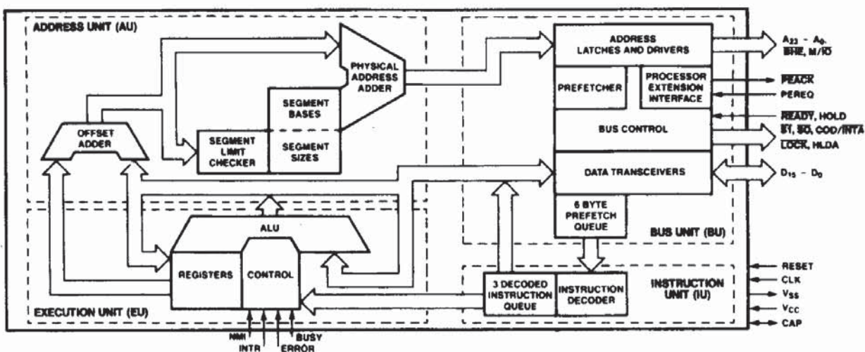
Figure 1. 80C286 Internal Block Diagram
