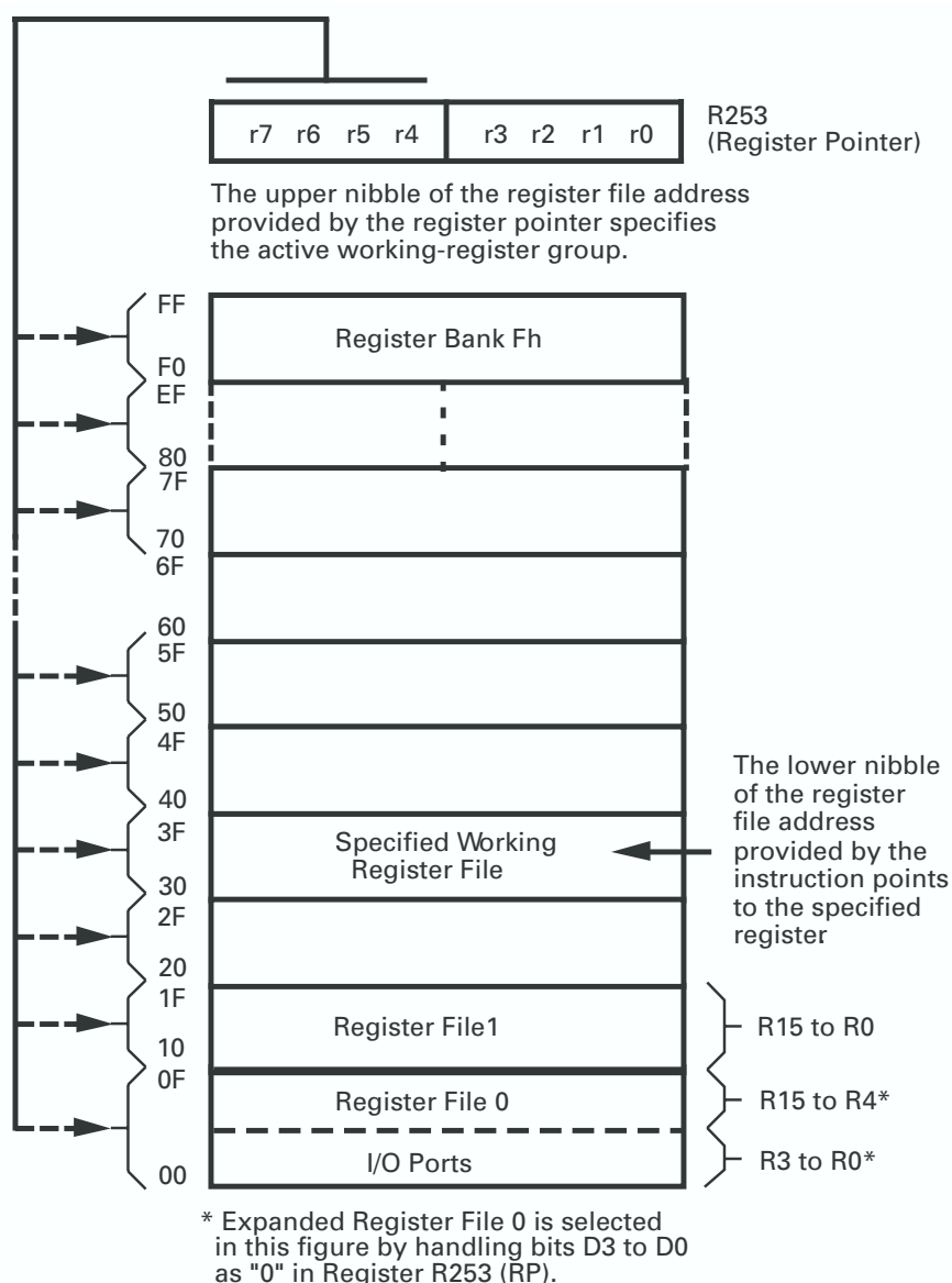
Figure 17. Register Pointer—Detail
