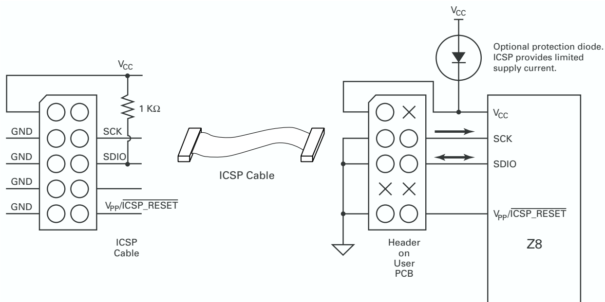
Figure 37. ICSP Connectivity
