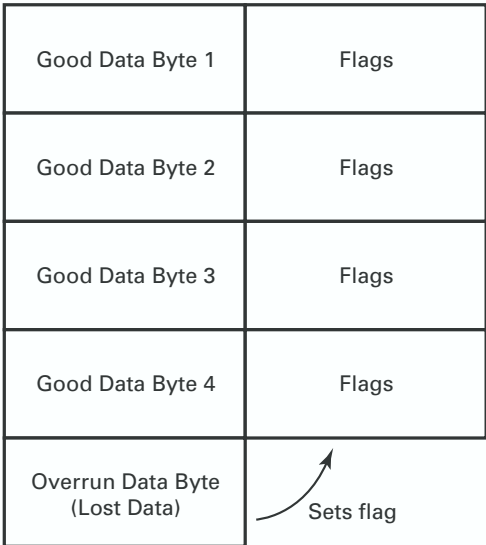
Figure 31. FIFO Overflow Example
