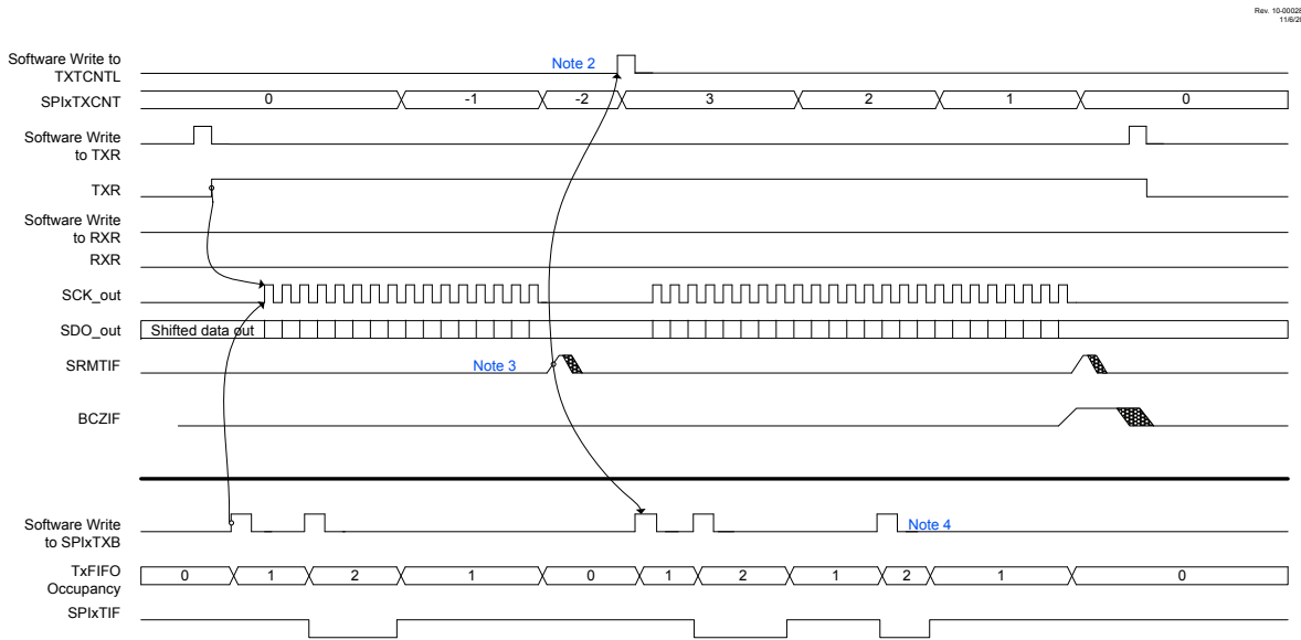
Figure 36-4. SPI Master Operation - Command+Write Data TXR = 1, RXR = 0
