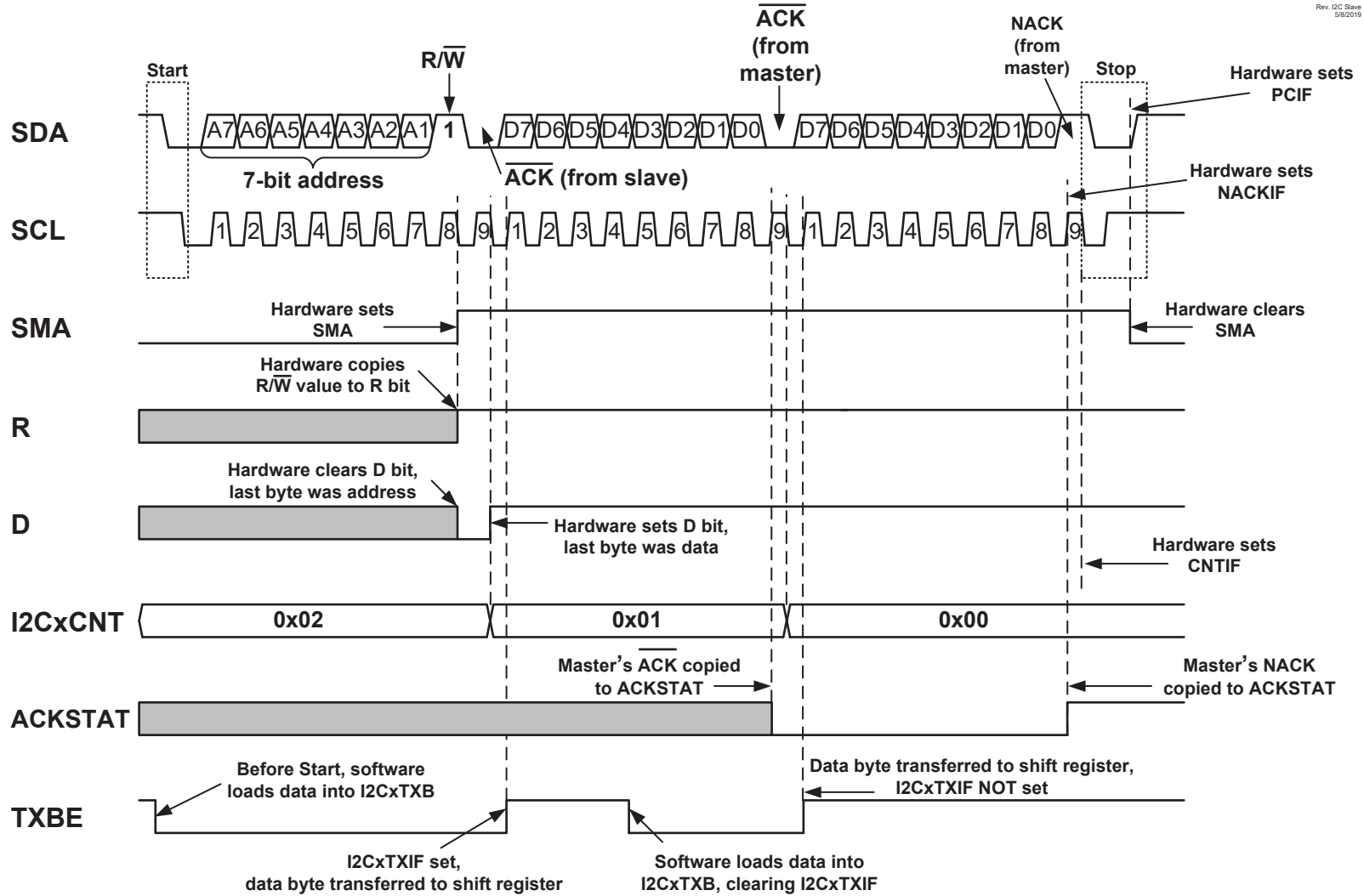
Figure 37-13. 7-Bit Slave Mode Transmission (No Clock Stretching)
