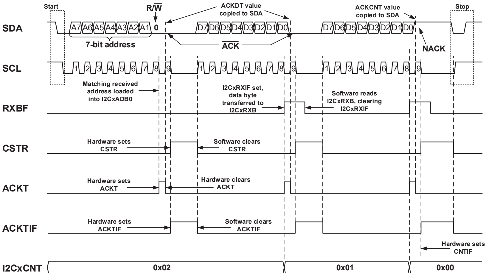
Figure 37-15. 7-Bit Slave Mode Transmission (ACKTIE = 1)
