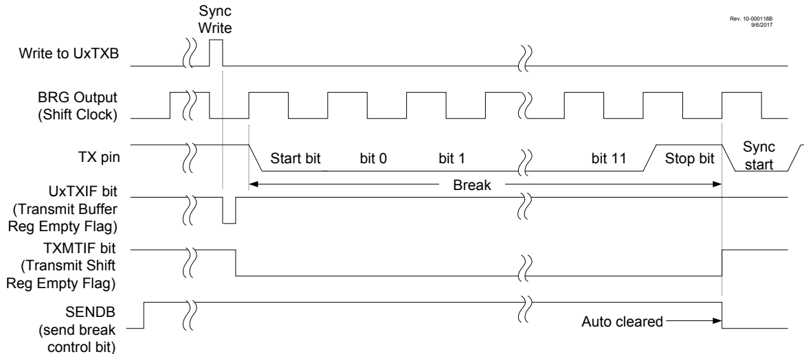
Figure 35-15. Send-Break Sequence
