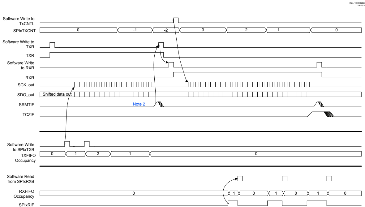
Figure 36-5. SPI Master Operation, Command+Read Data, TXR = 0, RXR = 1
