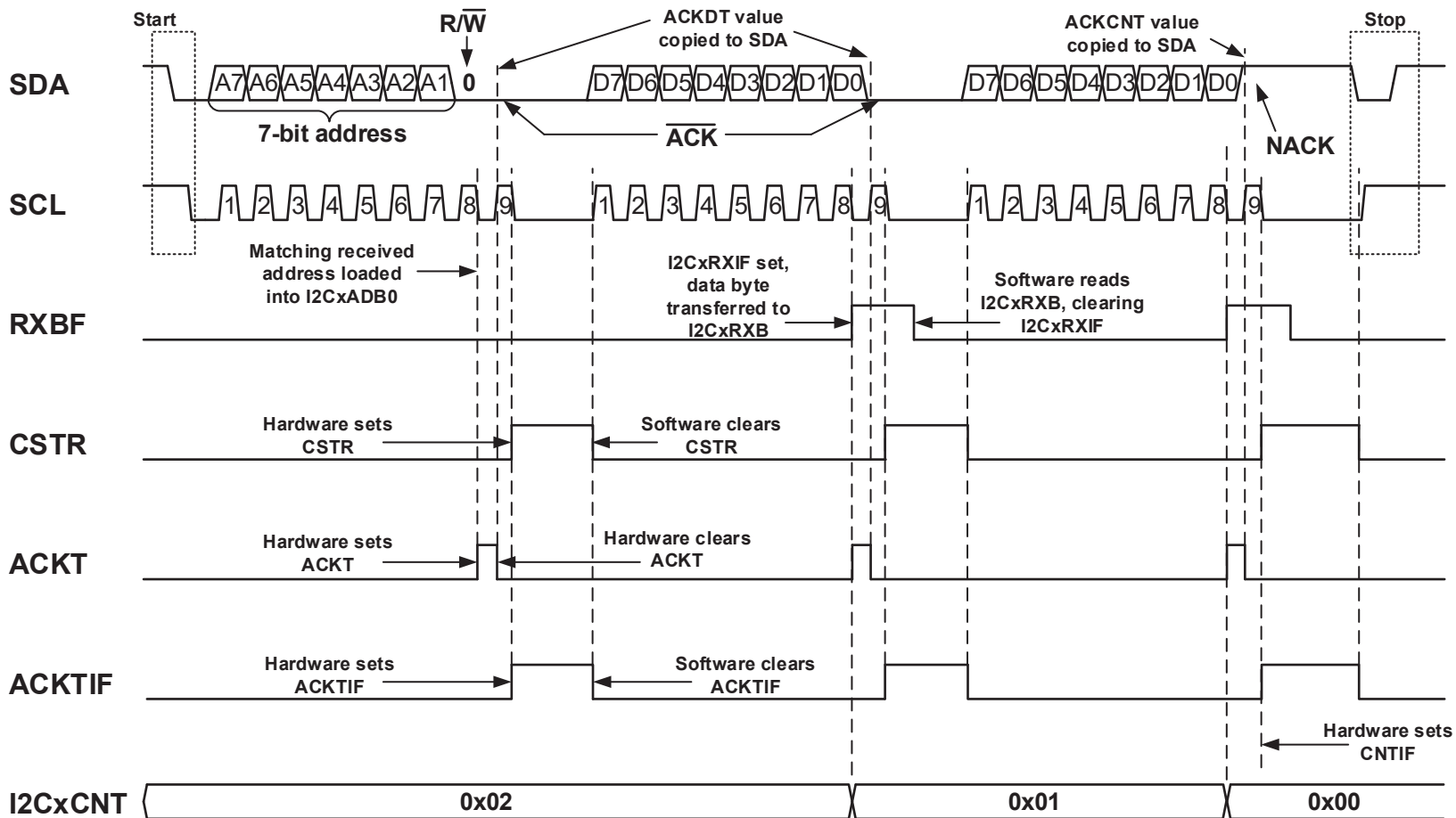
Figure 37-18. 7-Bit Slave Mode Reception (ACKTIE = 1)
