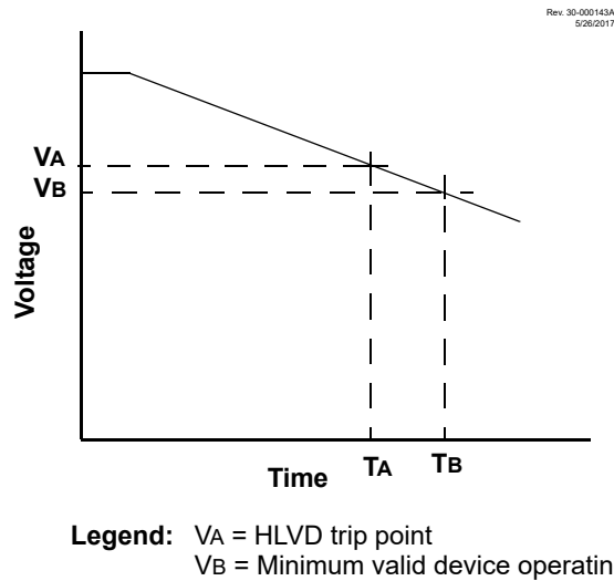
Figure 40-4. Typical Low-Voltage Detect Application
