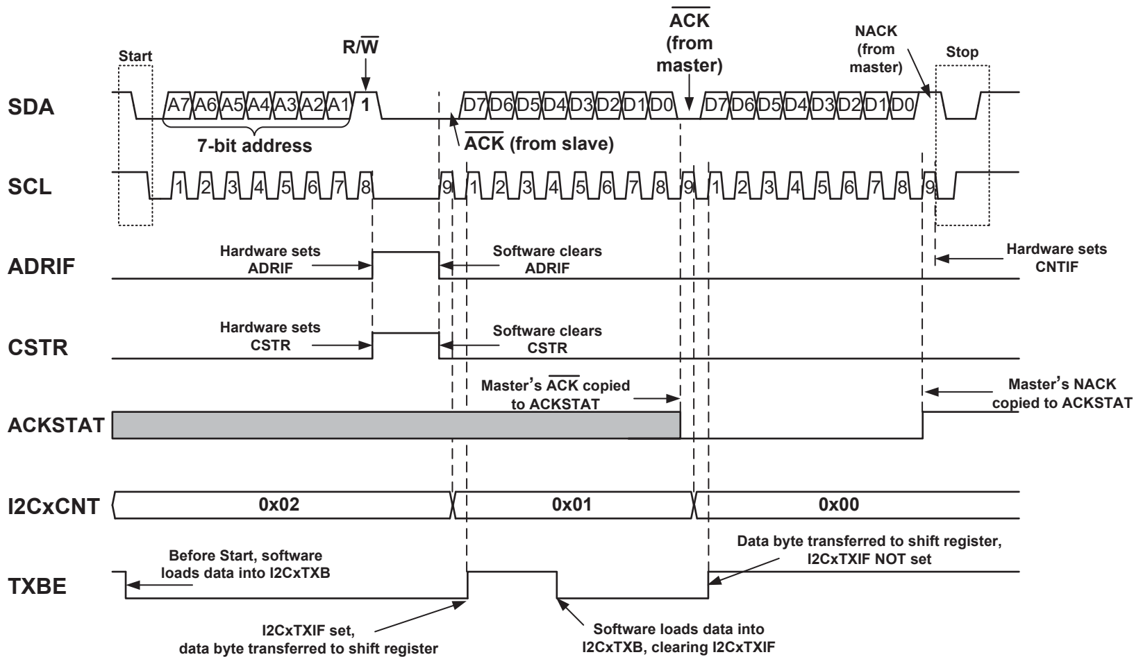
Figure 37-14. 7-Bit Slave Mode Transmission (ADRIE = 1)
