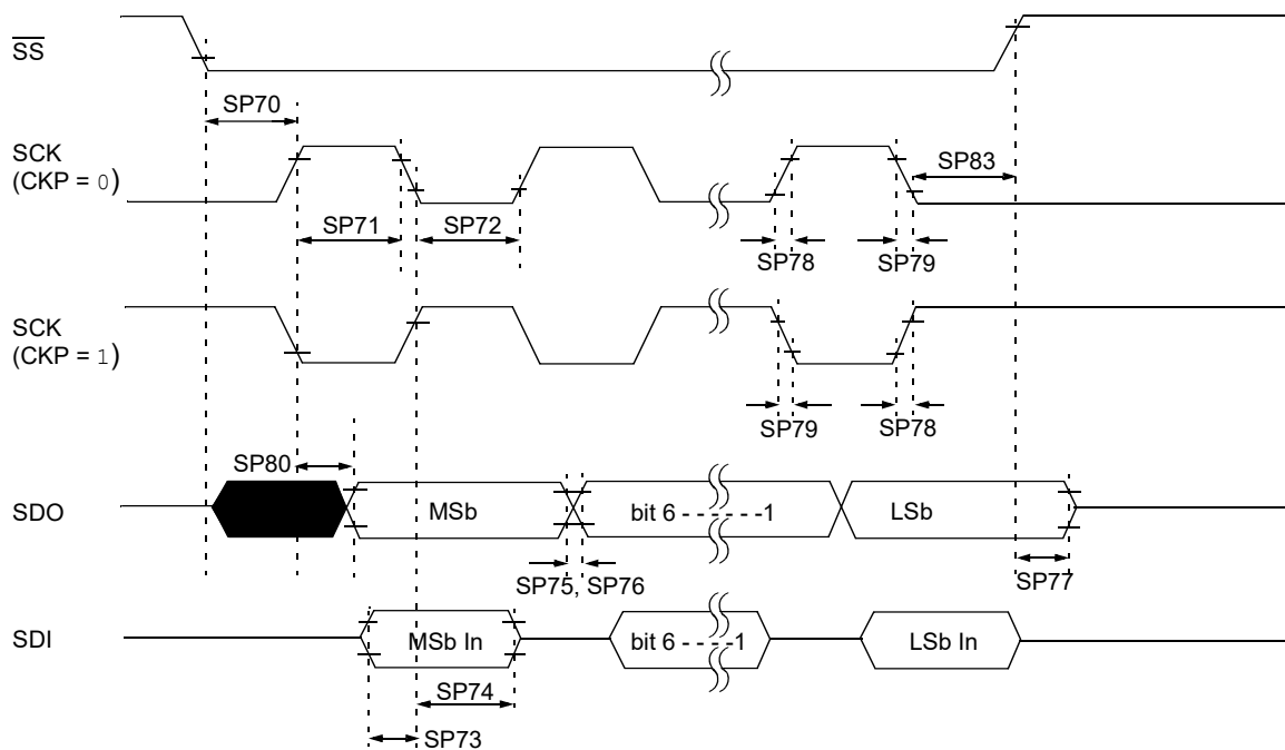
Figure 50-15. SPI Slave Mode Timing (CKE = 0)
