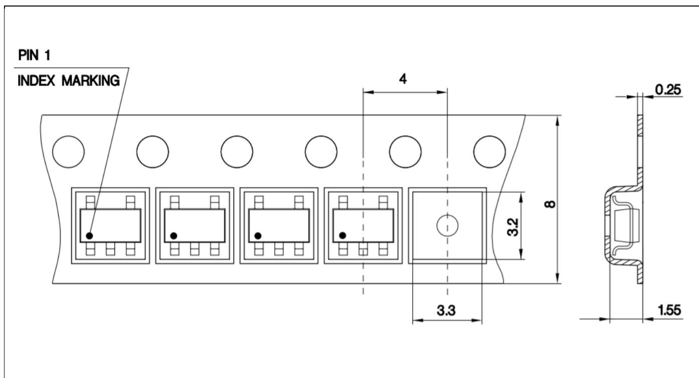
Figure 14 Tape and reel dimensions
