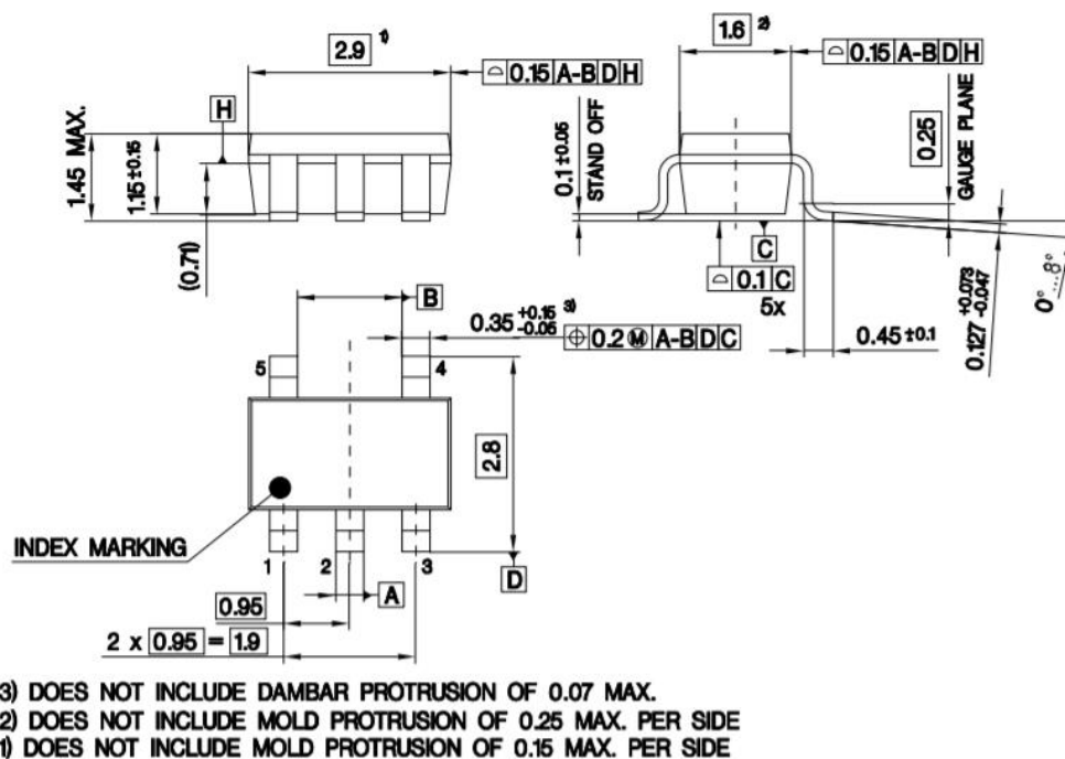
Outline dimensions
