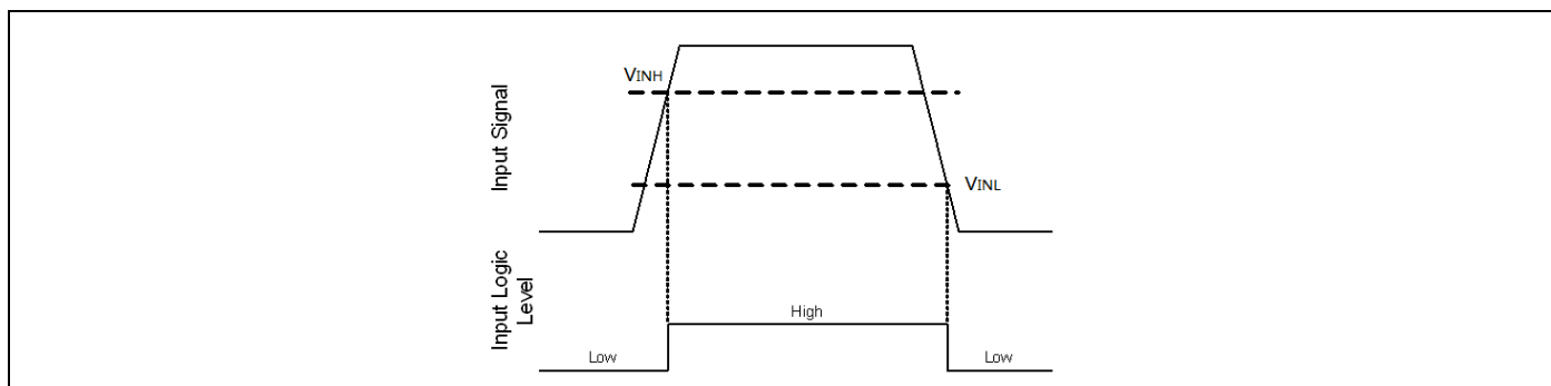
Figure 7 IN input thresholds
