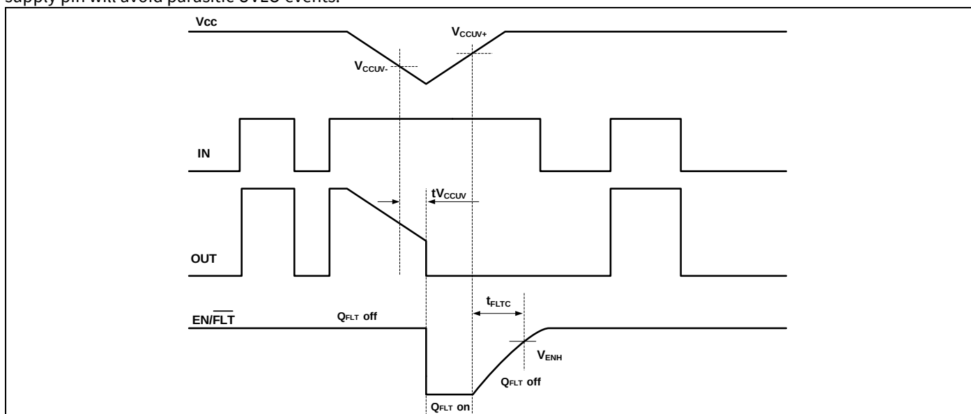
Figure 8 VCC under voltage protection waveform definitions
