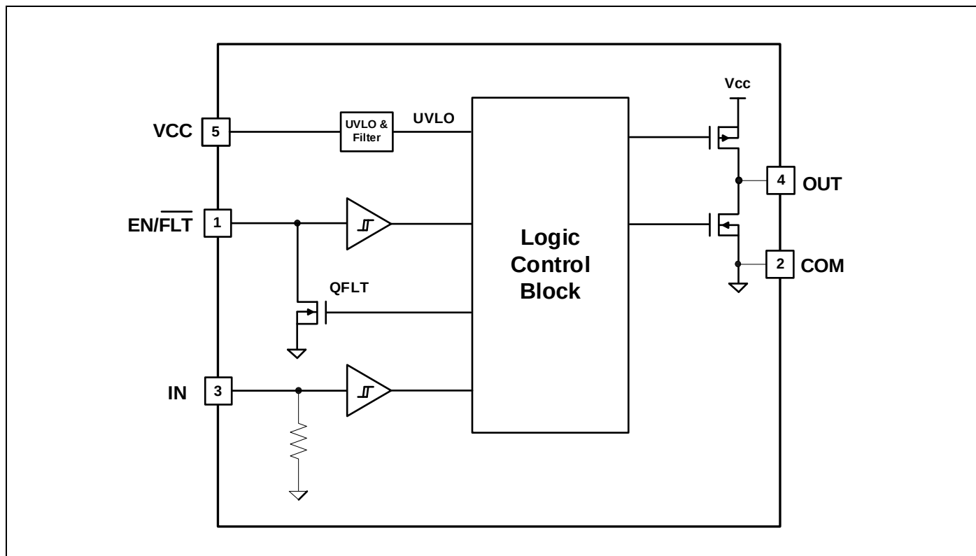
Figure 2 Block diagram
