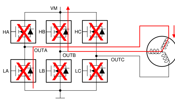
Figure 8-37. Coast State
