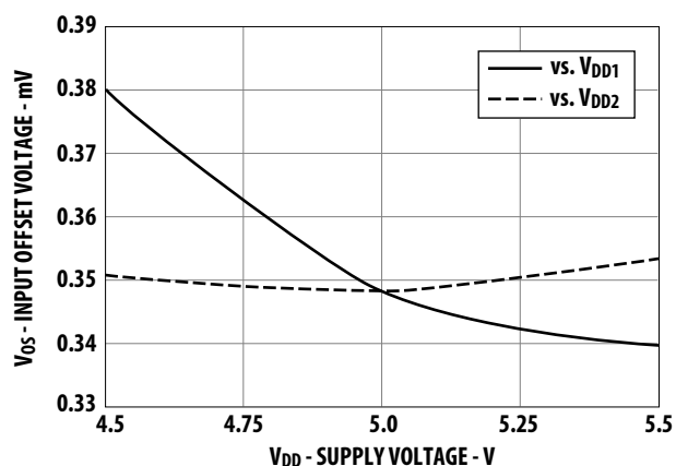
Figure 3: Input Offset Voltage vs. Supply Voltage
