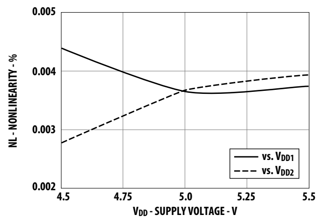
Figure 8: Nonlinearity vs. Supply Voltage
