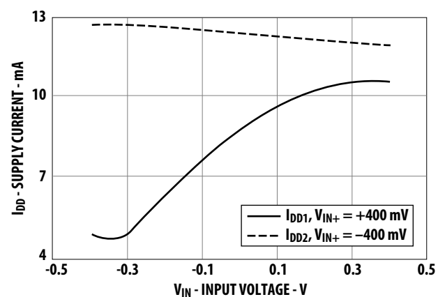
Figure 10: Supply Current vs. Input Voltage
