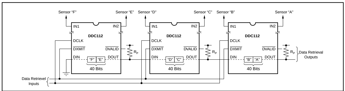
FIGURE 20. Daisy-Chained DDC112's.
