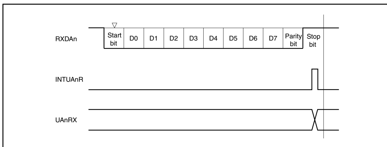
Figure 16-9. UART Reception
