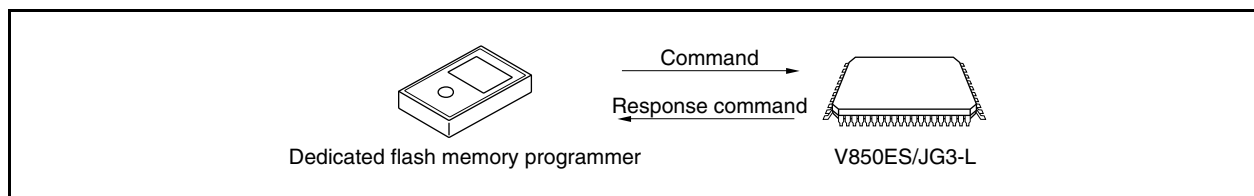
Figure 31-9. Communication Commands
