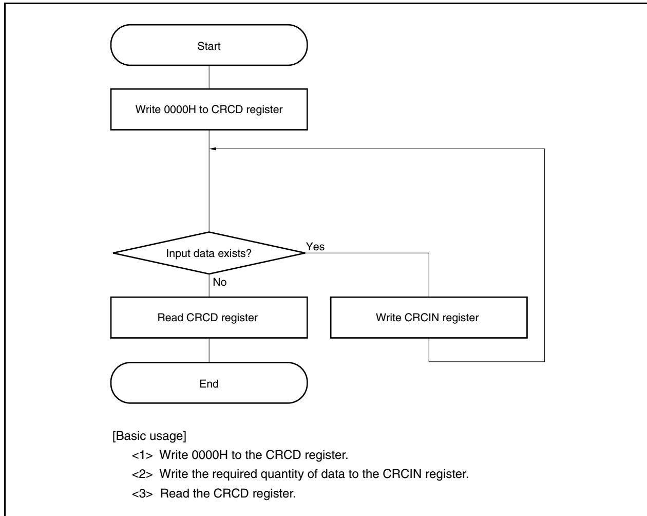
Figure 28-3. CRC Operation
