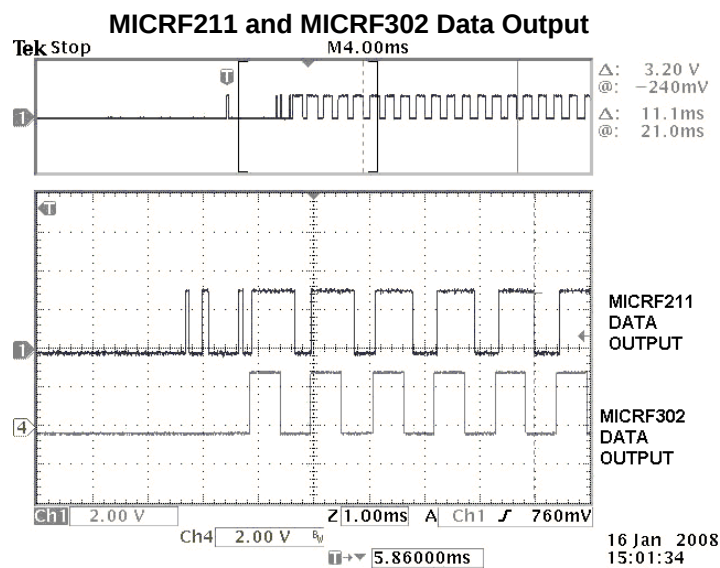
Figure 10. Micrel Receiver Example Receiving MICRF302 Data Output
