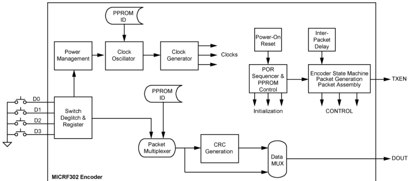
Figure 3. MICRF302 Parallel Encoder Functional Diagram
