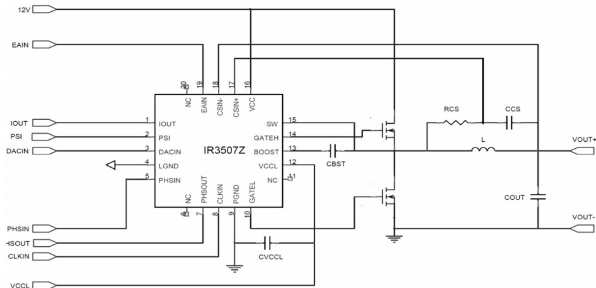
Figure 1 Application Circuit
