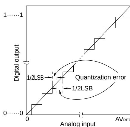
Figure 10-14. Quantization Error
