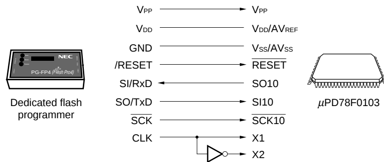
Figure 21-8. Communication with Dedicated Flash Programmer (CSI10)
