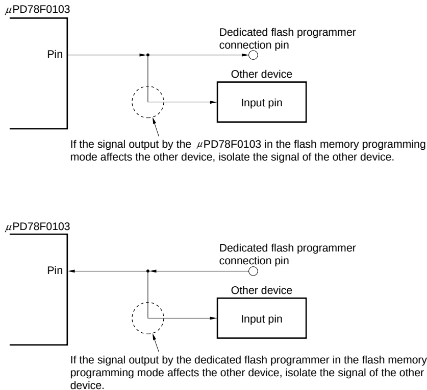
Figure 21-15. Malfunction of Other Device
