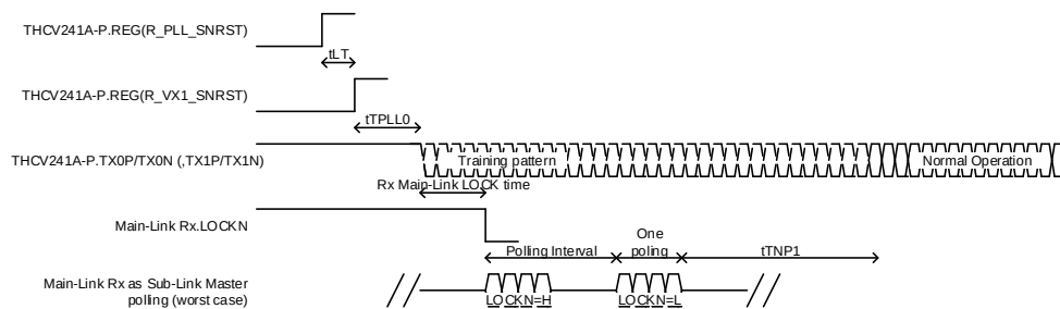
Figure 22. Lock Sequence
