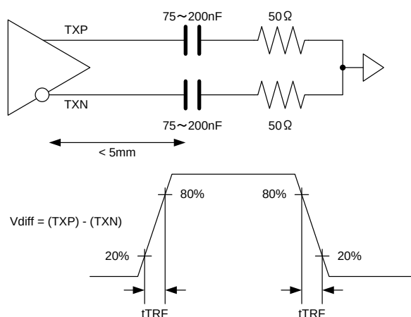
Figure 24. CML Transmitter tTRF
