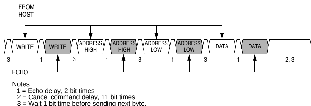
Figure 12-11. Write Transaction
