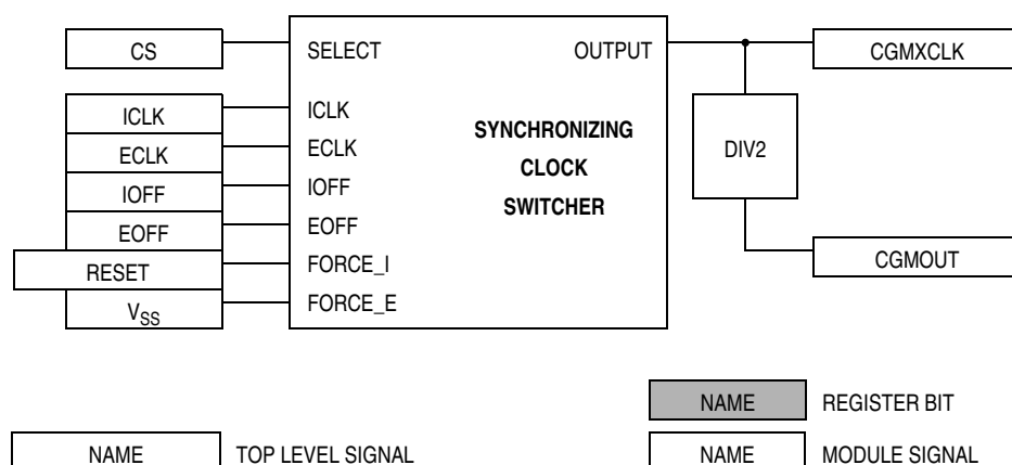
Figure 6-6. Clock Selection Circuit Block Diagram
