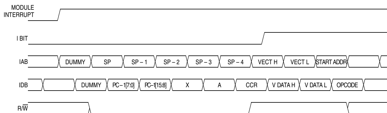
Figure 10-8. Interrupt Entry
