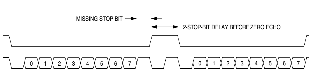
Figure 12-9. Break Transaction
