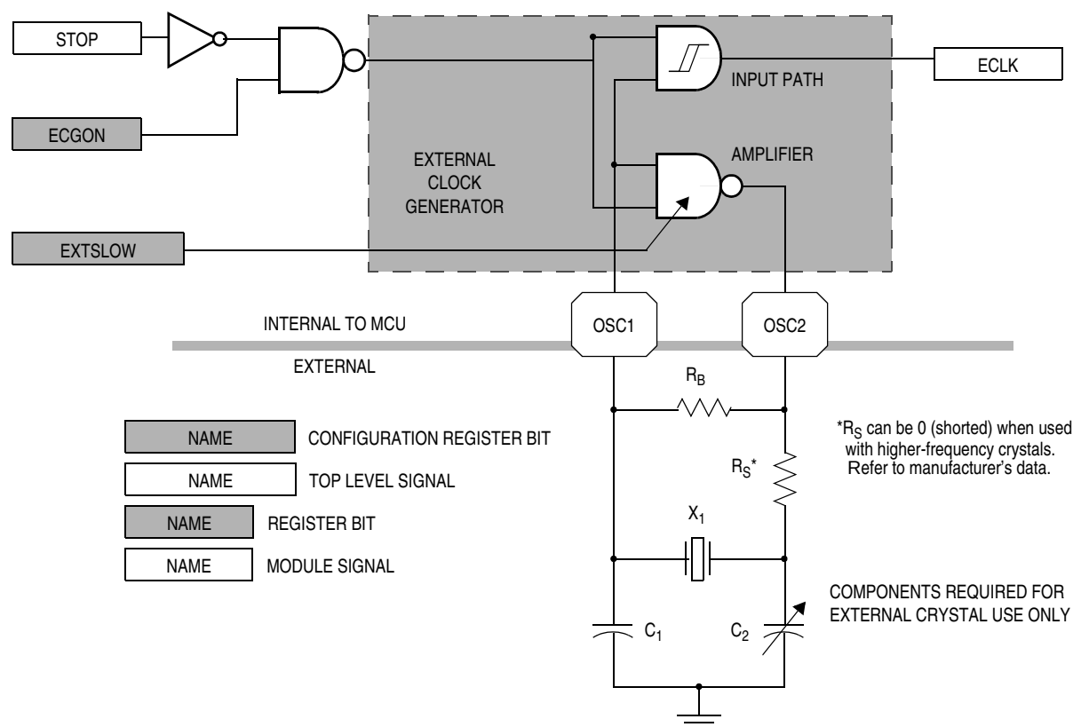
Figure 6-4. External Clock Generator Block Diagram
