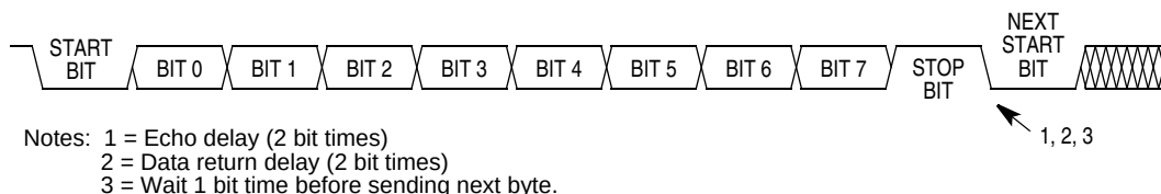
Figure 12-6. Monitor Data Format
