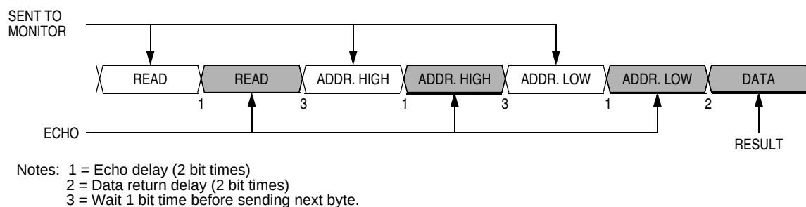
Figure 12-8. Read Transaction
