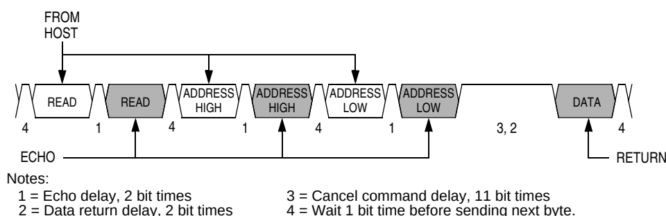
Figure 12-10. Read Transaction
