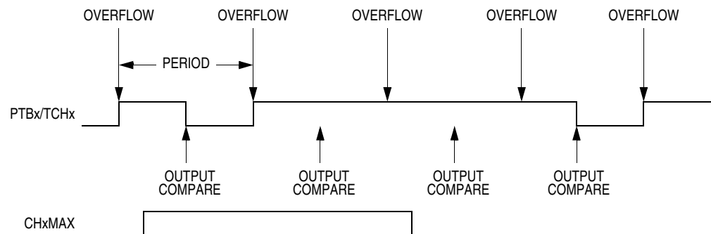
Figure 11-9. CHxMAX Latency
