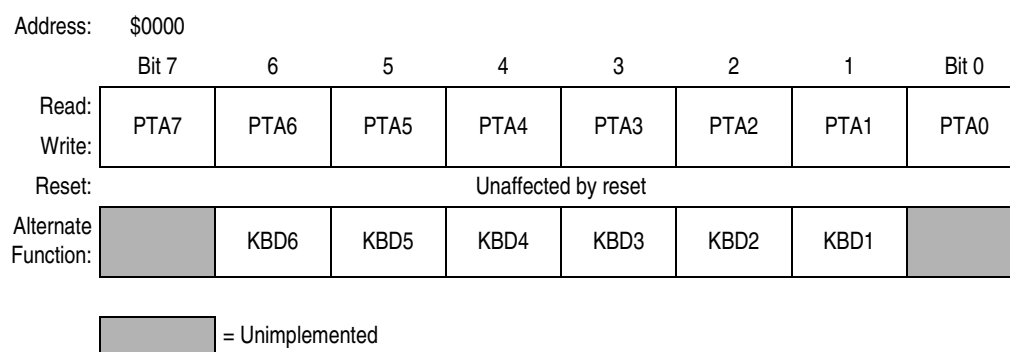
Figure 9-2. Port A Data Register (PTA)
