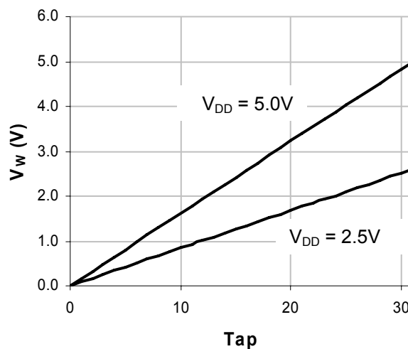
Wiper Voltage vs. Tap Position
