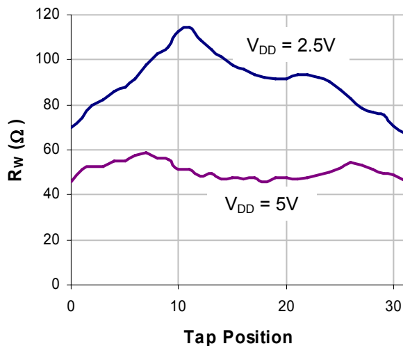
Wiper Resistance vs. Tap Position @ 25^\circ C
