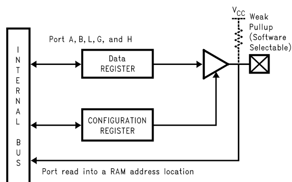
FIGURE 3. I/O Port Configurations
