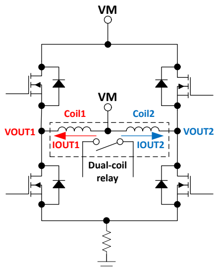
Figure 9-11. Schematic of dual-coil relay driven by the OUTx H-bridge
