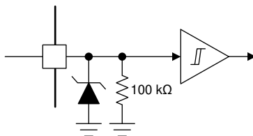
Figure 8-7. Logic-level input
