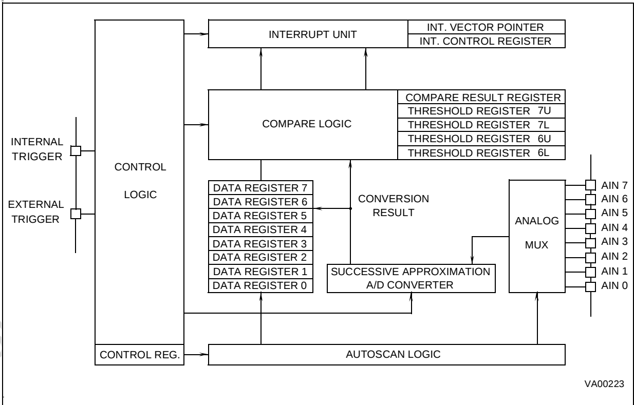
Figure 87. Block Diagram
