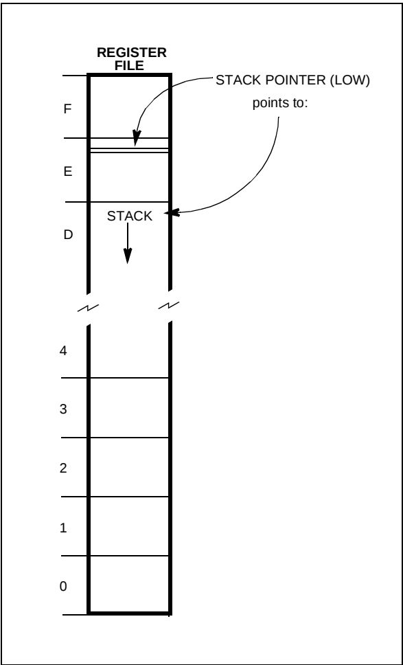
Figure 11. Internal Stack Mode
