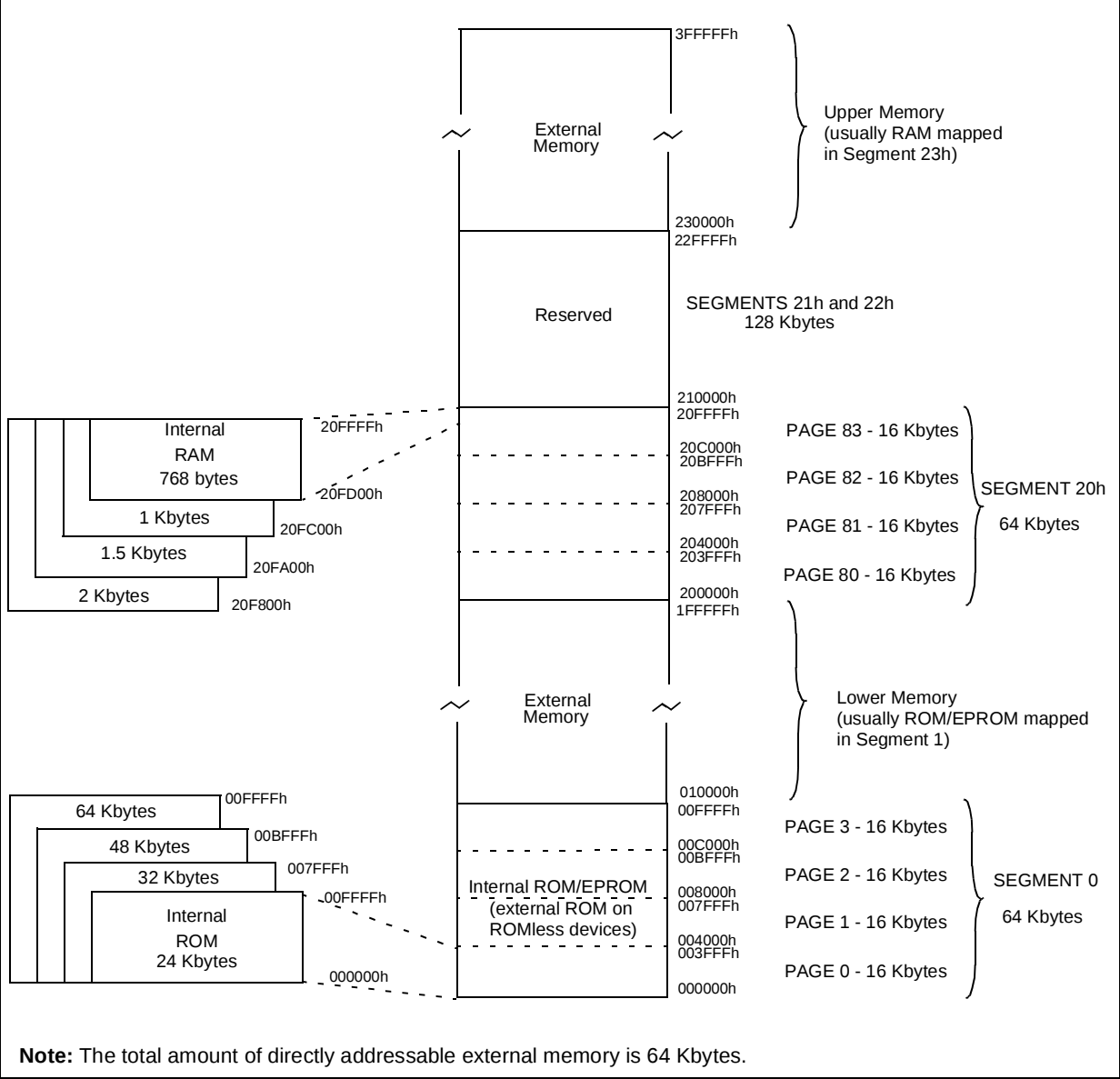
Figure 18. Memory Map
