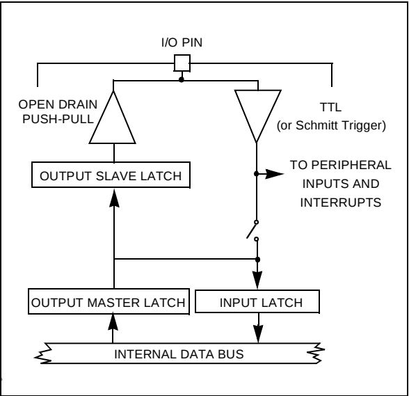
Figure 52. Output Configuration
