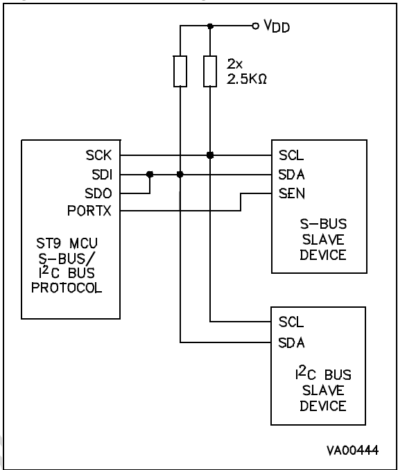
Figure 72. S-bus Configuration
