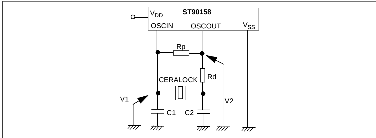
Figure 40. Test circuit
