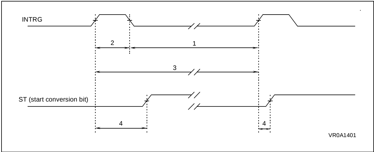
A/D INTERNAL TRIGGER TIMING
