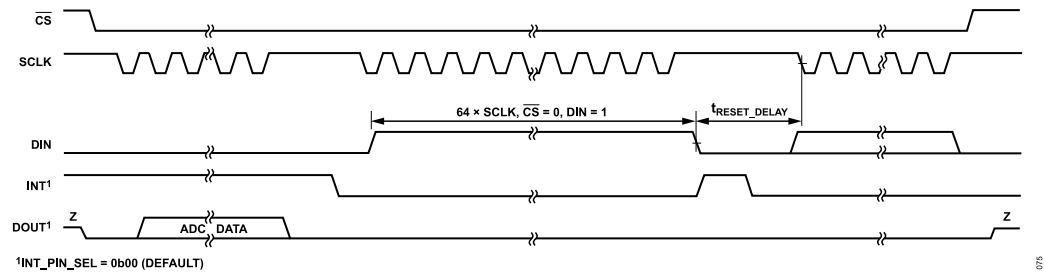
Figure 75. Software Reset Timing Diagram
