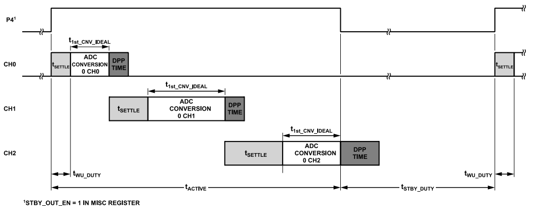
Figure 95. Example of Autonomous Duty Cycling Mode
