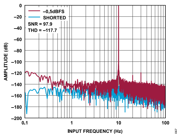
Figure 67. FFT, -0.5 dBFS vs. Shorted Inputs, 10 Hz Input Tone, \text{Sinc}^3 Filter, ODR = 240 SPS, Gain = 1, Internal Reference
