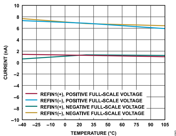
Figure 50. Reference Input Current vs. Temperature (Reference Buffer Bypass, External 2.5 V Reference)
