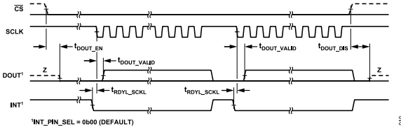
Figure 10. Continuous Read Mode Timing
