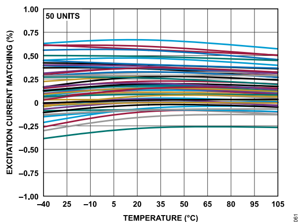
Figure 61. Excitation Current Matching vs. Temperature (100 \mu A)
