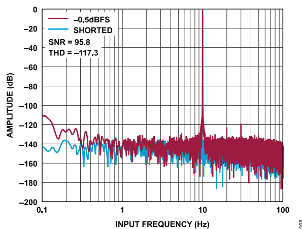
Figure 68. FFT, -0.5 dBFS vs. Shorted Inputs, 10 Hz Input Tone, \text{Sinc}^3 Filter, ODR = 240 SPS, Gain = 1, External Reference
