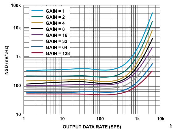
Figure 32. NSD vs. Output Data Rate for Various Gains ( \text{Sinc}^3 Filter, External 2.5 V Reference)
