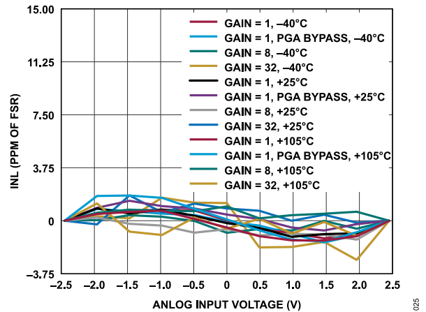
Figure 25. INL Error vs. VIN/Gain for Various Gains and Temperatures (Sinc 3 Filter, ODR = 50 SPS, External 2.5 V Reference)
