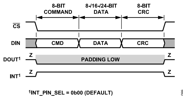
Figure 99. SPI Write Transaction with CRC
