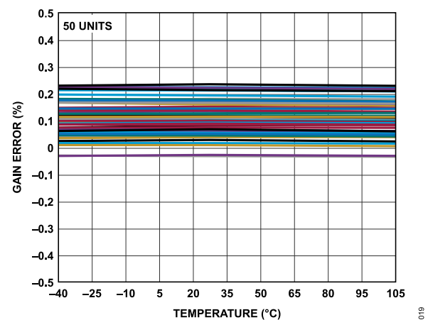
Figure 19. Gain Error vs. Temperature (Gain = 8, Before Calibration)
