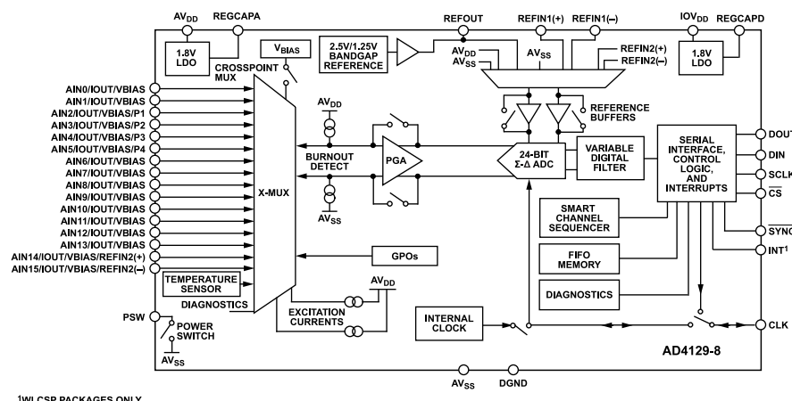
Figure 69. Detailed Block Diagram
