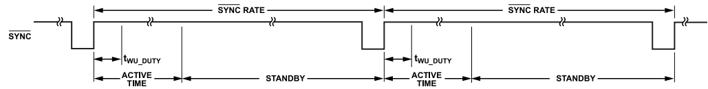
Figure 79. Example of Single Sequence + STBY by SYNC Mode Diagram
