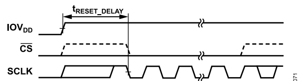
Figure 71. POR Timing Diagram
