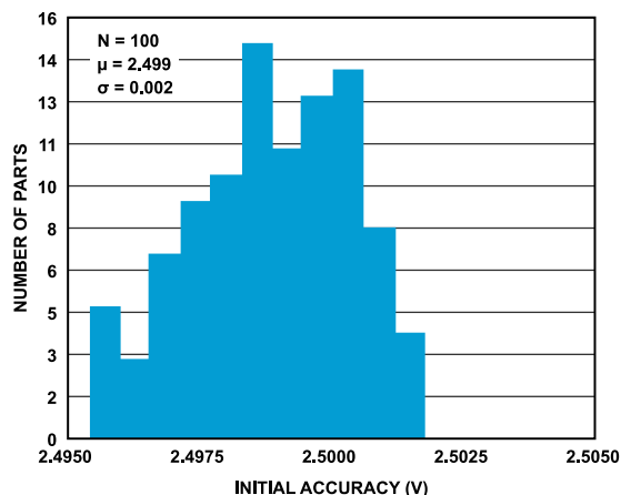
Figure 51. 2.5 V Internal Reference Voltage Histogram
