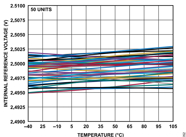
Figure 52. 2.5 V Internal Reference Voltage vs. Temperature
