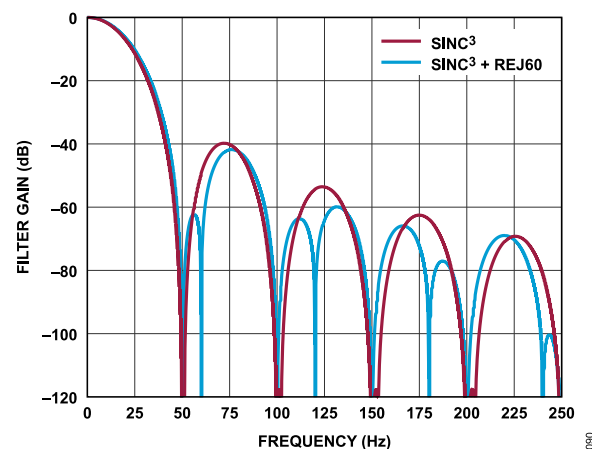
Figure 90. Sinc 3 and Sinc 3 + REJ60 Filter Response (50 SPS ODR)
