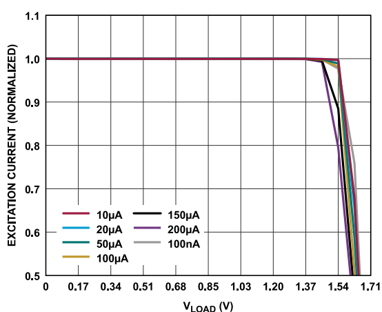
Figure 62. Output Compliance for Various IEXC Sources ( AV_{DD} = 1.71 V)
