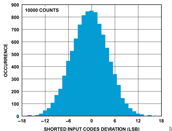
Figure 27. Noise Histogram Plot ( \text{Sinc}^3 Filter, ODR = 50 SPS, Gain = 1)
