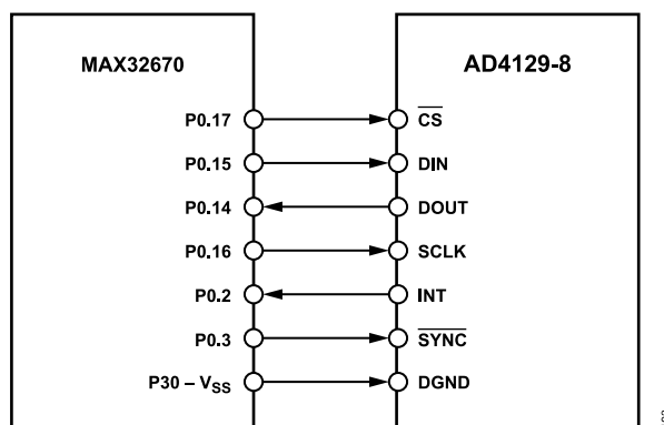
Figure 107. Example of MAX32670 \mu C SPI Connection to AD4129-8
