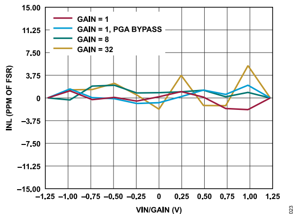
Figure 23. INL Error vs. VIN/Gain for Various Gains (Sinc 3 Filter, ODR = 50 SPS, AV DD = 1.8 V, Internal 1.25 V Reference)
