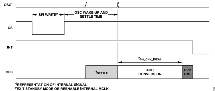
Figure 96. Out of Standby Mode Diagram
