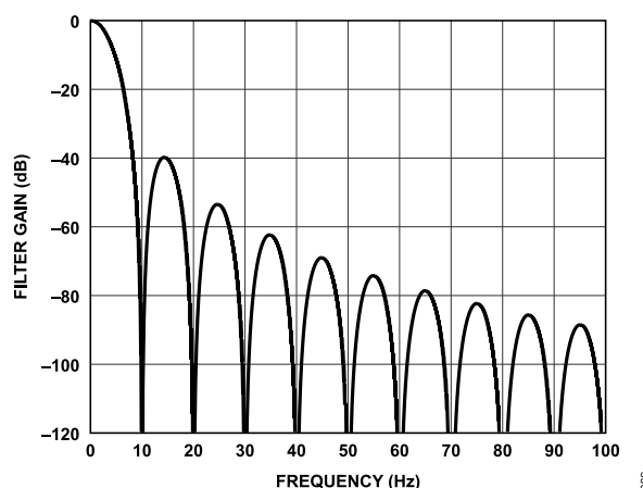
Figure 89. Simultaneous 50 Hz and 60 Hz Rejection for Sinc 3 with ODR = 10 SPS
