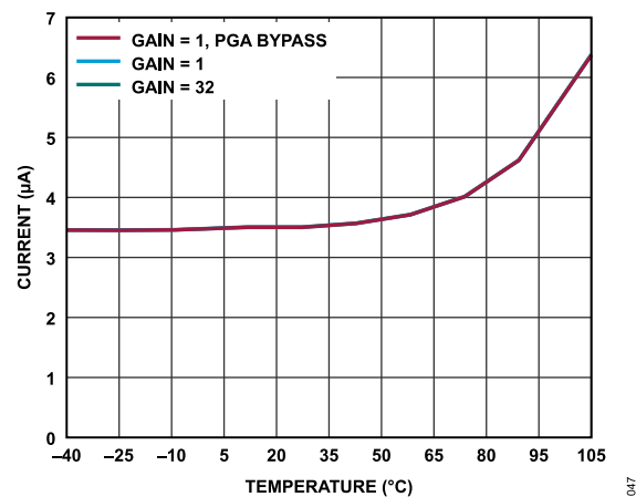
Figure 47. IOV_{DD} Current vs. Temperature
