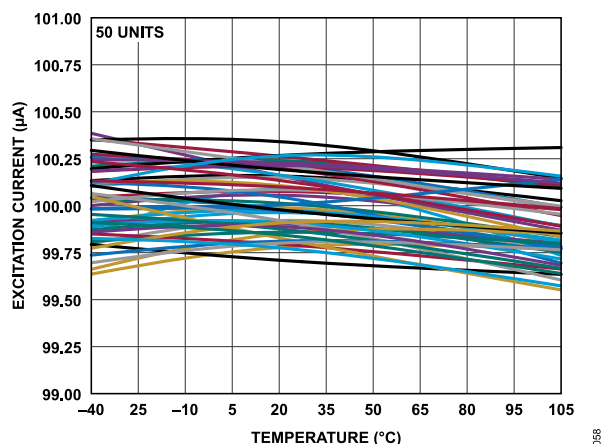
Figure 58. Excitation Current vs. Temperature (100 \mu A)
