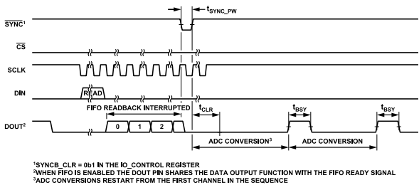
Figure 13. FIFO Clear Timing Diagram
