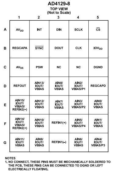
Figure 14. Pin Configuration
