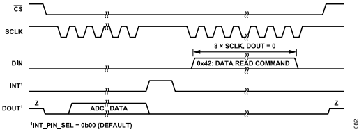
Figure 82. Exit Continuous Read Mode Diagram (CRC Disabled)
