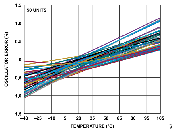
Figure 26. Internal Oscillator Error vs. Temperature
