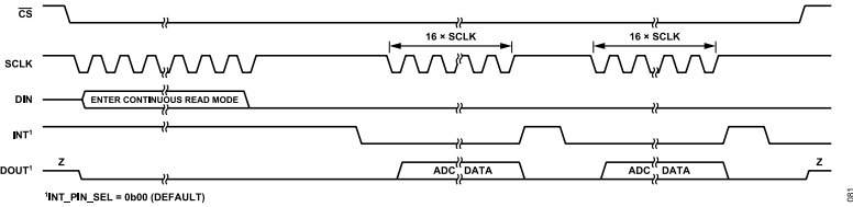
Figure 81. Enter Continuous Read Mode Diagram ( DATA\_STATUS = 0 )
