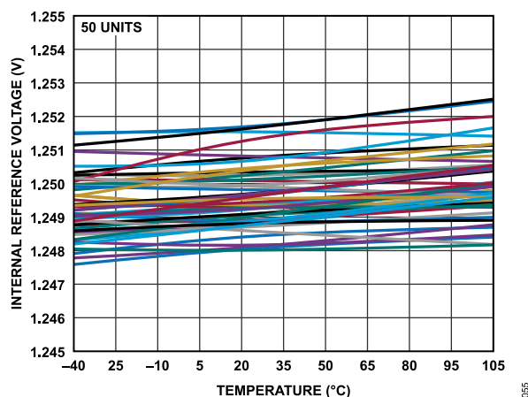
Figure 55. 1.25 V Internal Reference Voltage vs. Temperature
