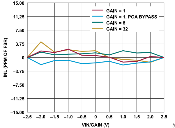
Figure 21. INL Error vs. Differential Input Amplitude (VIN/Gain) for Various Gains (Sinc 3 Filter, ODR = 50 SPS, Internal 2.5 V Reference)
