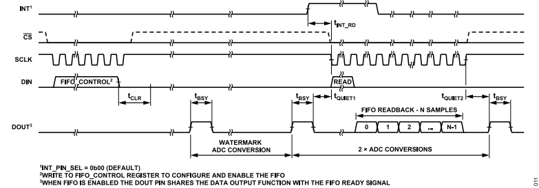
Figure 11. FIFO Timing with Watermark Interrupt
