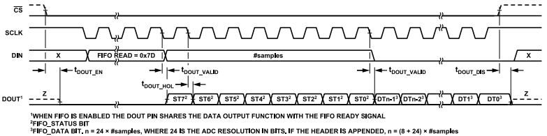
Figure 12. FIFO Readback Timing Diagram
