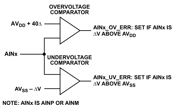
Figure 98. Analog Input Overvoltage/Undervoltage Monitors
