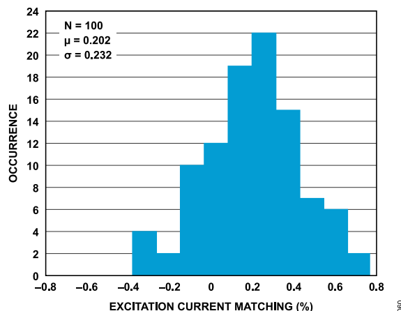
Figure 60. Excitation Current Initial Matching Histogram (100 \mu A)
