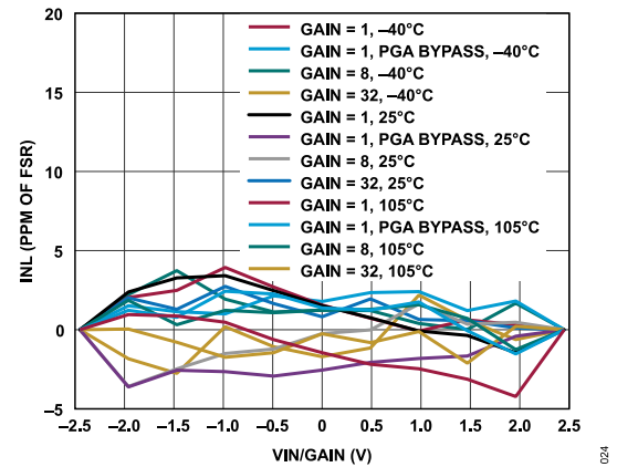
Figure 24. INL Error vs. VIN/Gain for Various Gains and Temperatures (Sinc 3 Filter, ODR = 50 SPS, Internal 2.5 V Reference)
