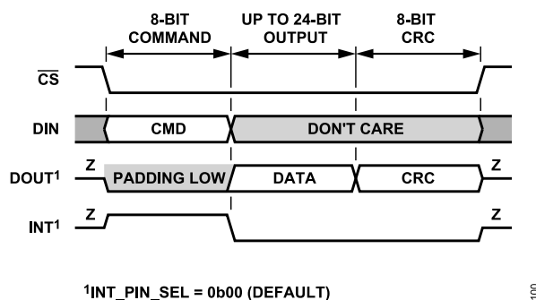
Figure 100. SPI Read Transaction with CRC
