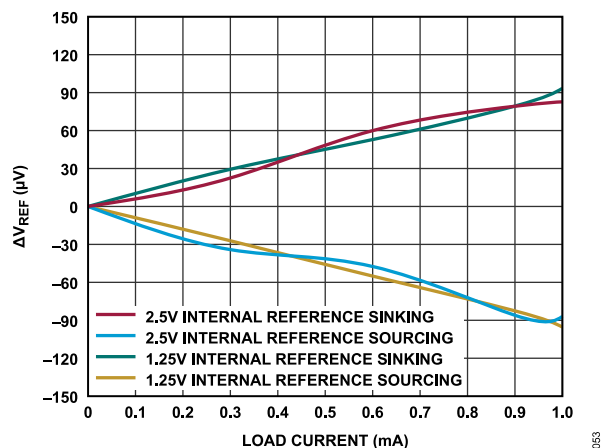
Figure 53. 1.25 V ( AV_{DD} = 1.8 V) and 2.5 V ( AV_{DD} = 3.3 V) Internal Reference Voltage vs. Load Current
