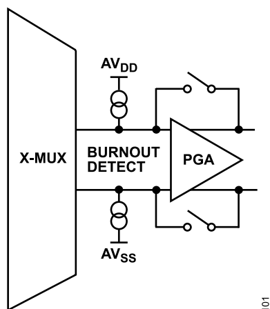
Figure 101. Burnout Currents
