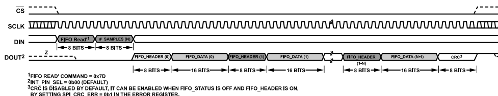
Figure 106. FIFO Readback (FIFO_STATUS Append Off and FIFO_HEADER Append On, CRC On)
