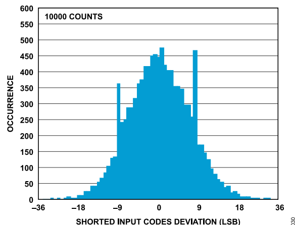
Figure 30. Noise Histogram Plot ( \text{Sinc}^4 Filter, ODR = 240 SPS, Gain = 1, Internal 1.25 V Reference)
