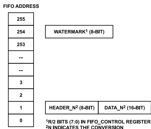
Figure 102. FIFO Structure
