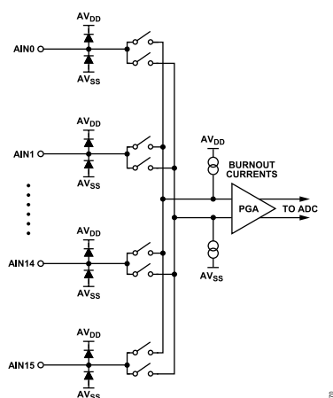
Figure 70. Analog Input Multiplexer Circuit
