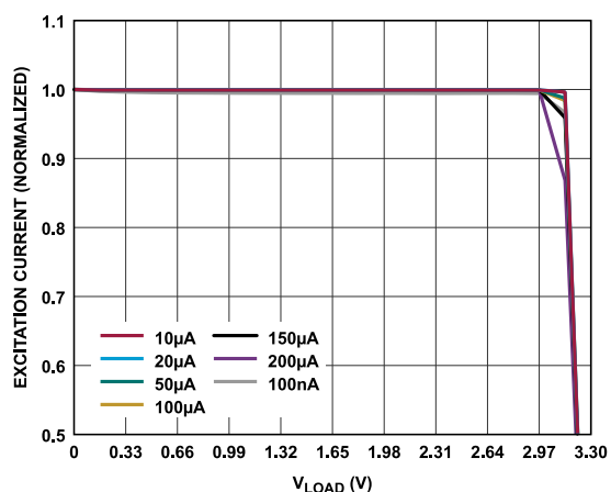
Figure 59. Output Compliance for Various IEXC Sources ( AV_{DD} = 3.3 V, V_{LOAD} is Load Voltage)
