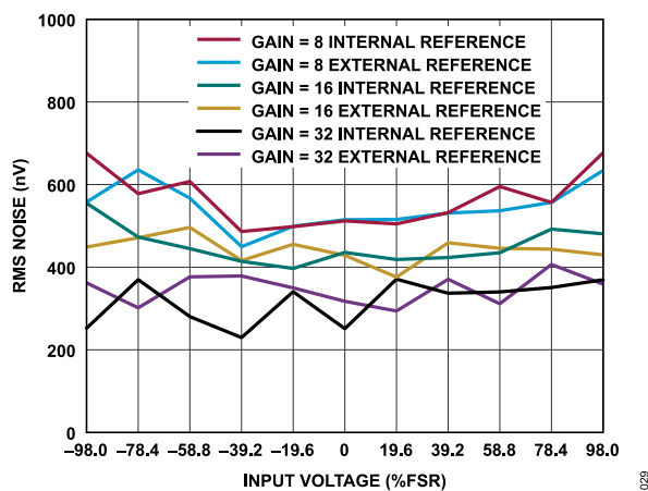
Figure 29. RMS Noise vs. Analog Input Voltage ( \text{Sinc}^3 Filter, ODR = 50 SPS, Gain = 8, Gain = 16 and Gain = 32, 1.25 V Reference)
