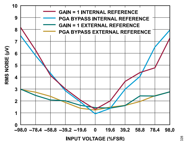
Figure 28. RMS Noise vs. Analog Input Voltage ( \text{Sinc}^3 Filter, ODR = 50 SPS, Gain = 1 and Gain = 1 with PGA Bypass, 2.5 V Reference)
