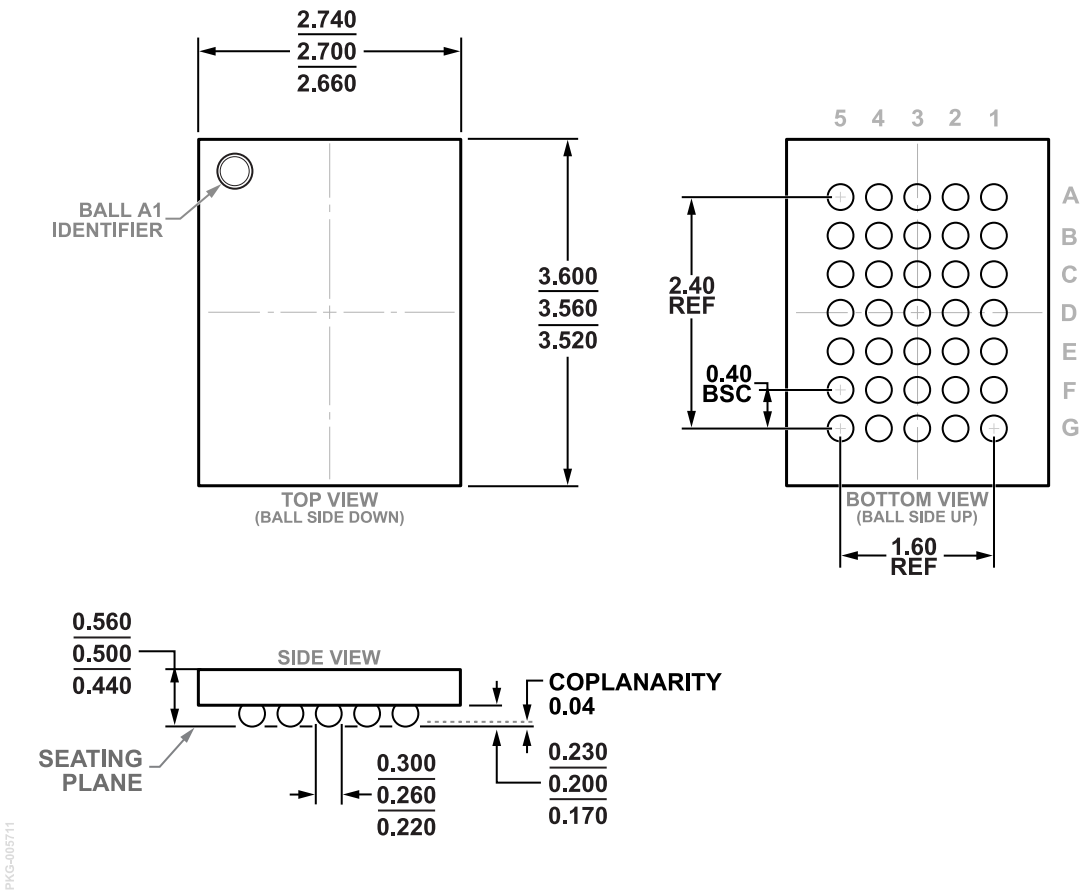
Figure 127. 35-Ball Wafer Level Chip Scale Package [WLCSP] 2.7 mm × 3.56 mm Body and 0.5 mm Package Height (CB-35-3) Dimensions Shown in Millimeters
