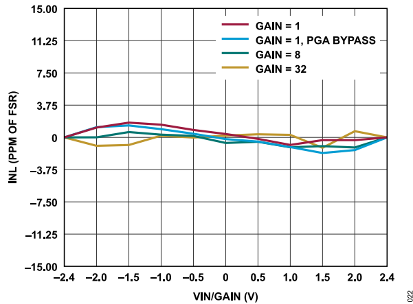
Figure 22. INL Error vs. VIN/Gain for Various Gains (Sinc 3 Filter, ODR = 50 SPS, External 2.5 V Reference)
