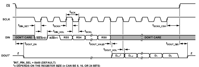
Figure 6. 3-Wire Mode Read Cycle Timing Diagram, 3-Wire Mode (CSB_EN Bit Set to 0), \overline{CS} Pin Used to Tristate the DOUT Pin
