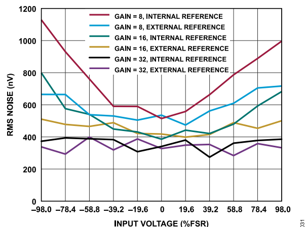
Figure 31. RMS Noise vs. Analog Input Voltage ( \text{Sinc}^3 Filter, ODR = 50 SPS, Gain = 8, Gain = 16 and Gain = 32, 2.5 V Reference)
