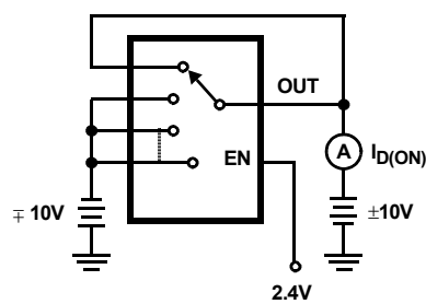
FIGURE 4. I_{D(ON)} TEST CIRCUIT (NOTE 8)
