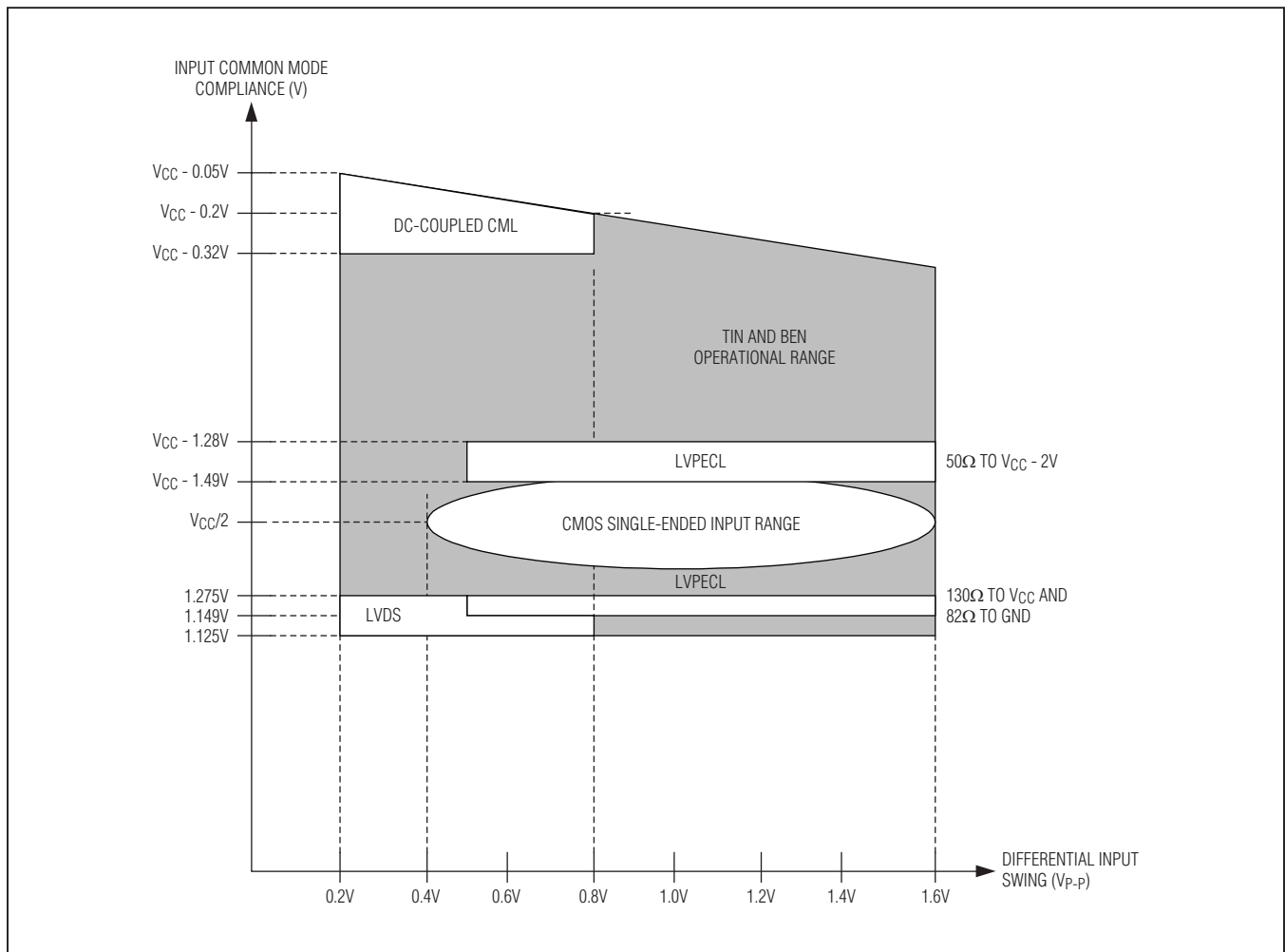
Figure 1. BEN/TIN Input Voltage Diagram
