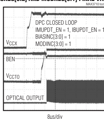
LASER STARTUP WITH PRECONDITIONING (SET_IBIAS[7:0] AND SET_IMOD[7:0] LOADED WITH VALUES CLOSE TO BIASREG[9:2] AND MODREG[8:1] FINAL VALUES)
