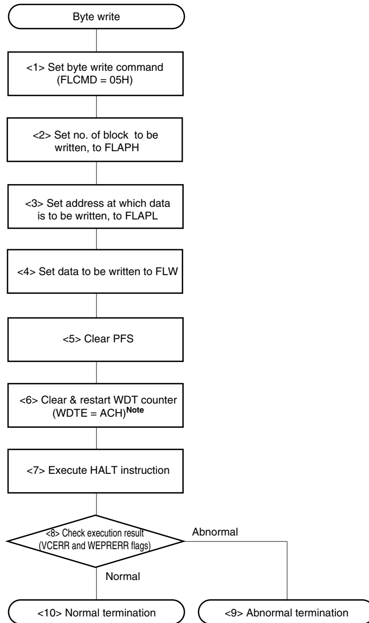
Figure 15-24. Example of Byte Write Operation in Self Programming Mode
