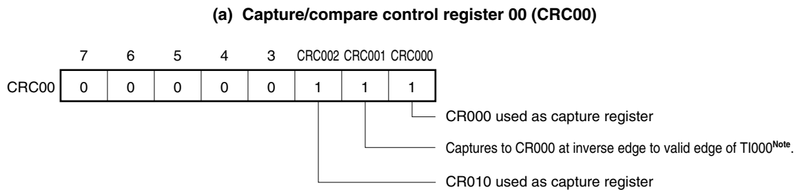
Figure 6-25. Control Register Settings for Pulse Width Measurement by Means of Restart (with Rising Edge Specified) (1/2)
