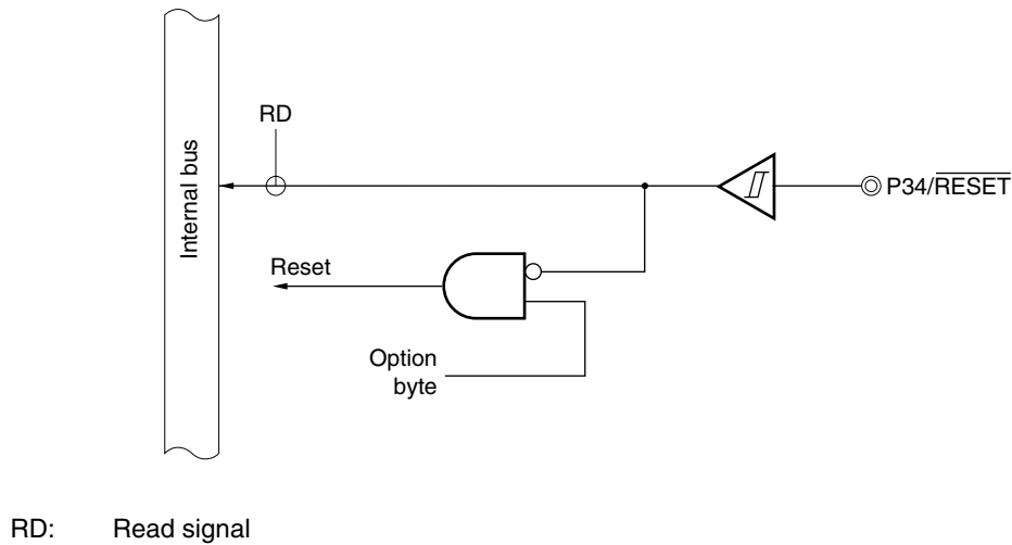
Figure 4-6. Block Diagram of P34
