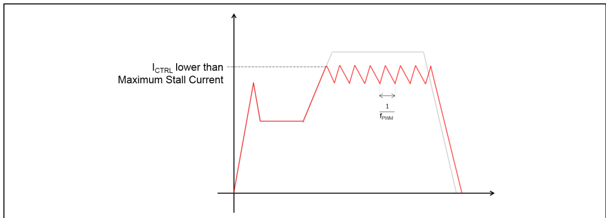
Figure 7. Slightly regulated door lock current
