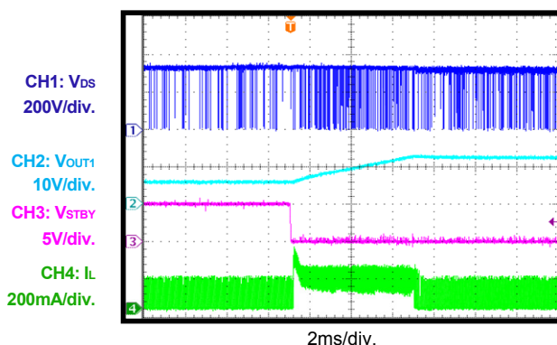
Standby Recovery I_{OUT1} = 0A , I_{OUT2} = 50mA
