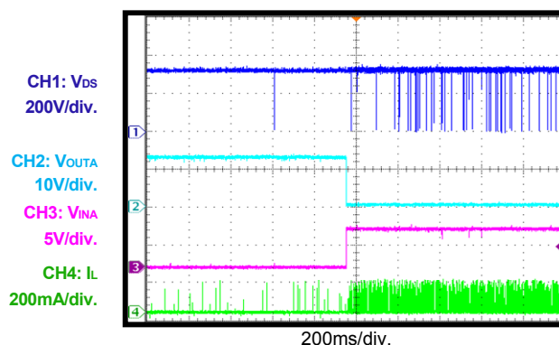
Relay 1 Turn-On No Load
