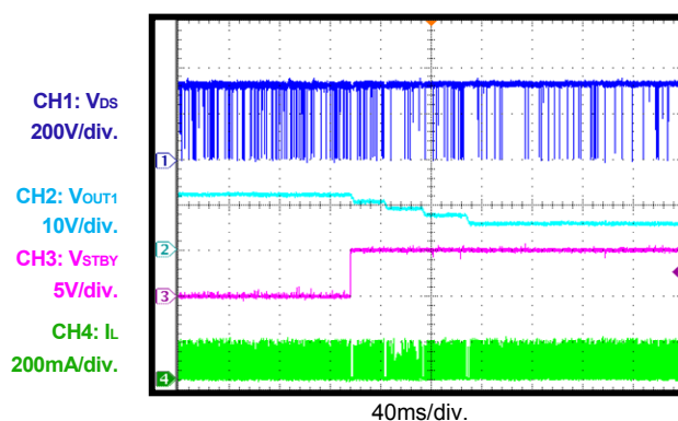
Standby Entry I_{OUT1} = 0A , I_{OUT2} = 50mA
