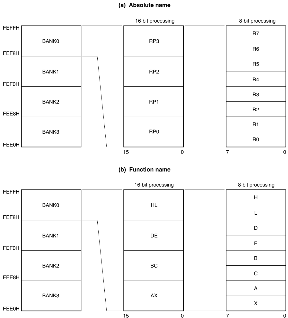
Figure 3-10. Configuration of General-Purpose Registers
