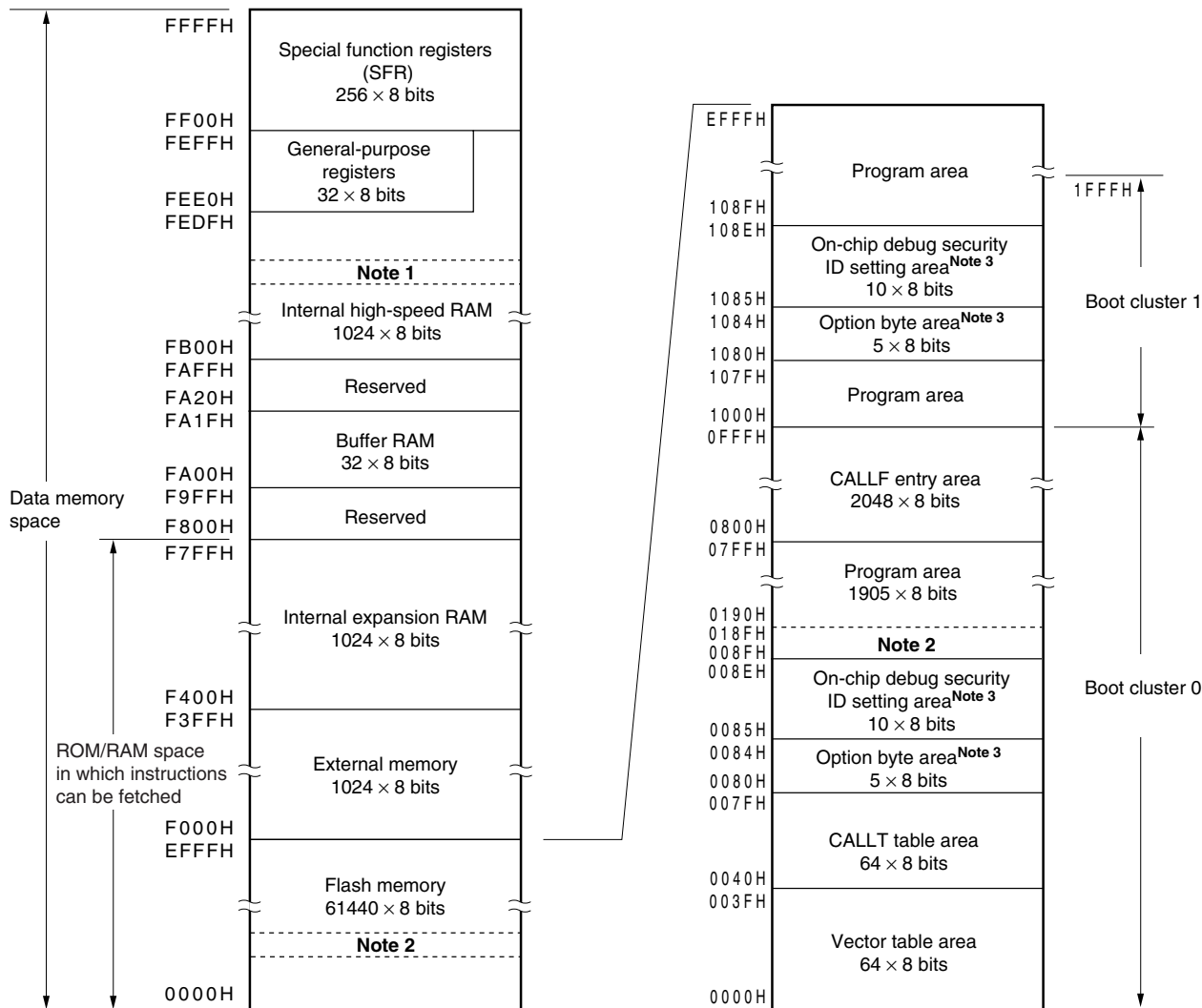
Figure 3-2. Memory Map (μPD78F0148HD)
