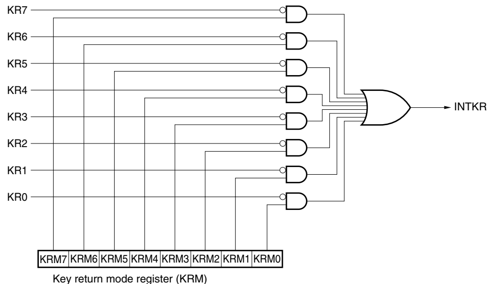
Figure 20-1. Block Diagram of Key Interrupt
