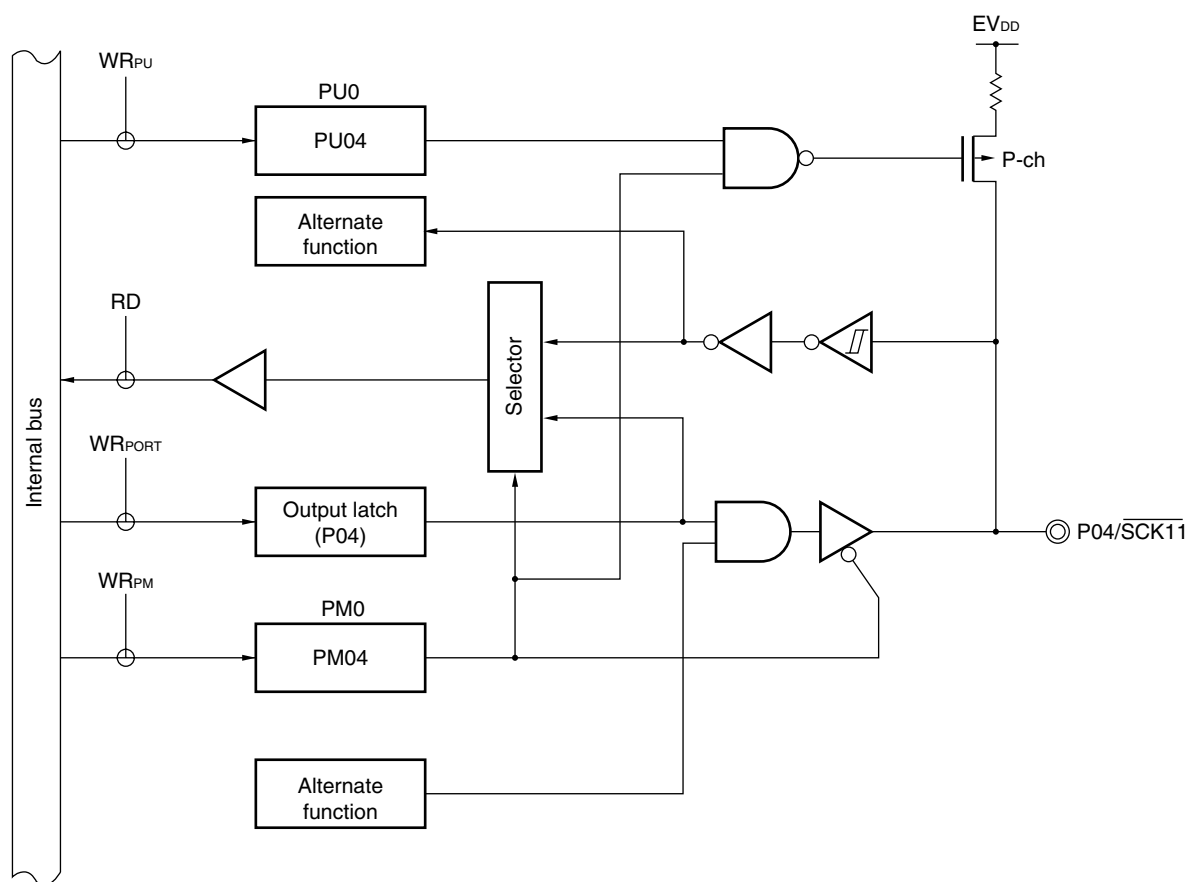
Figure 4-5. Block Diagram of P04
