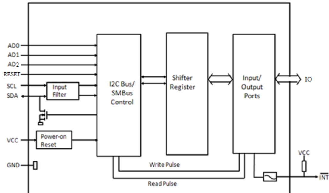
Fig 2: Block diagram
