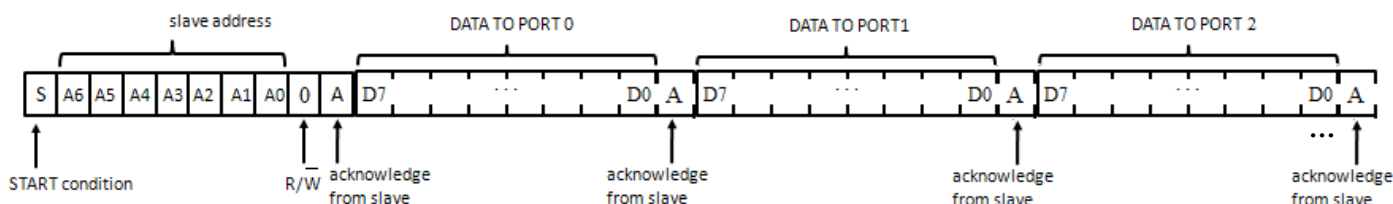
Fig 4. Write Mode
