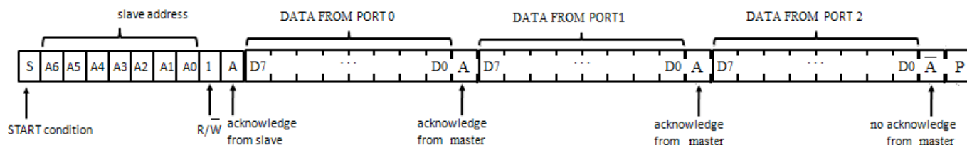
Fig 5. Read input port register
