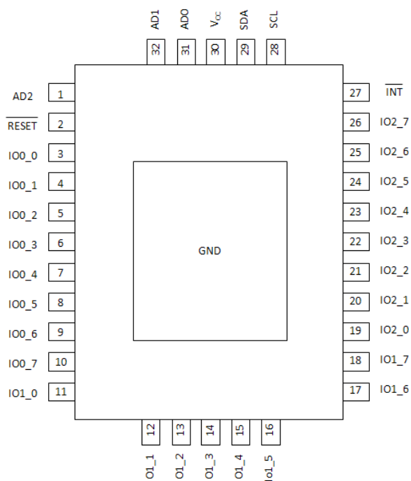
Fig 1 Pin Assignment
