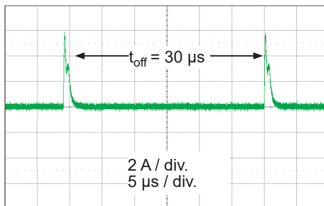
Figure 7. Short-to-load event
