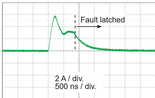
Figure 6. Short-to-ground event
