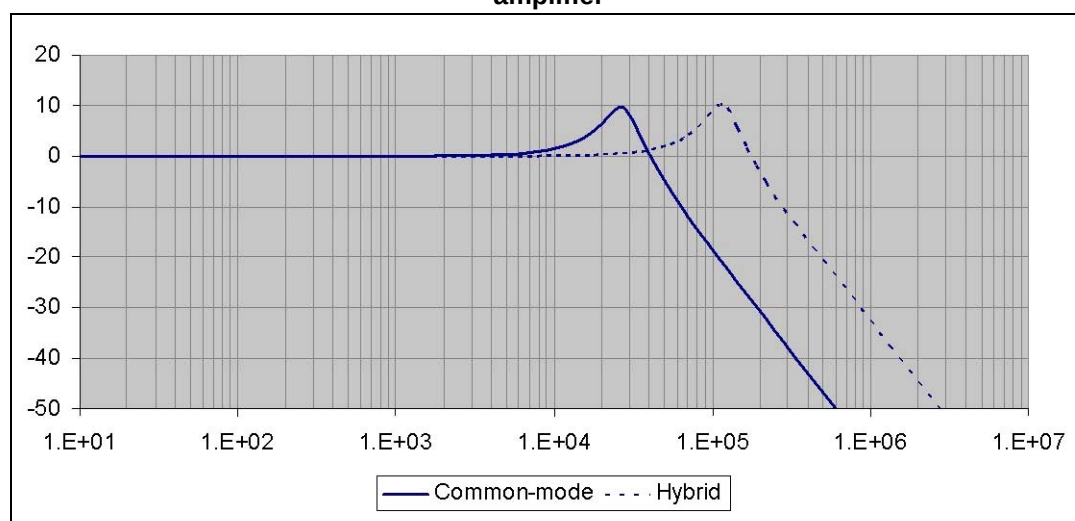
Figure 23. Output filter frequency response with and without load connected to the amplifier
