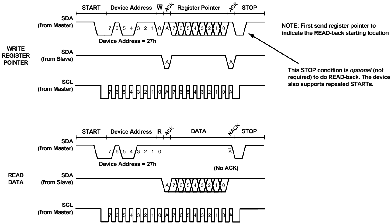
FIGURE 21. I 2 C READ TIMING DIAGRAM
