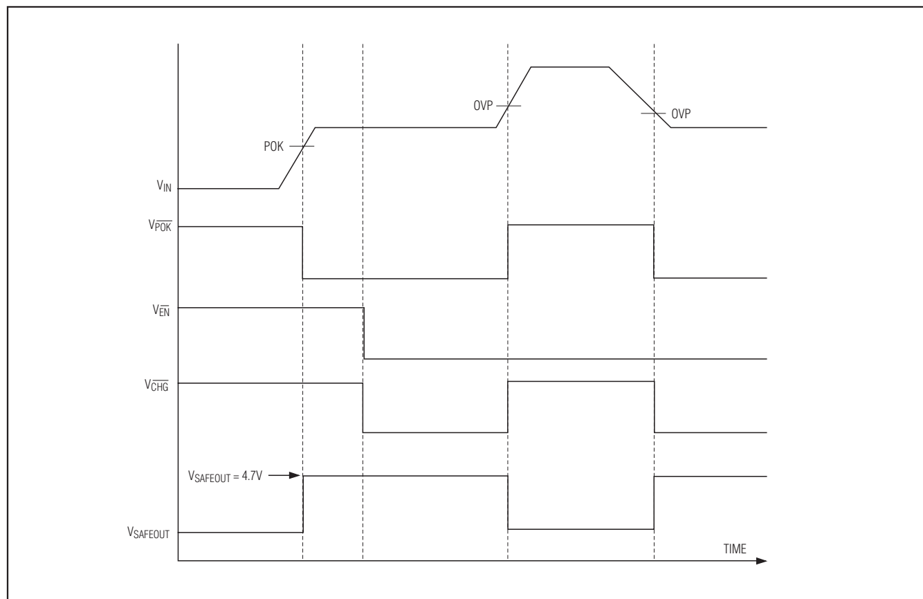
Figure 6. Timing Diagram
