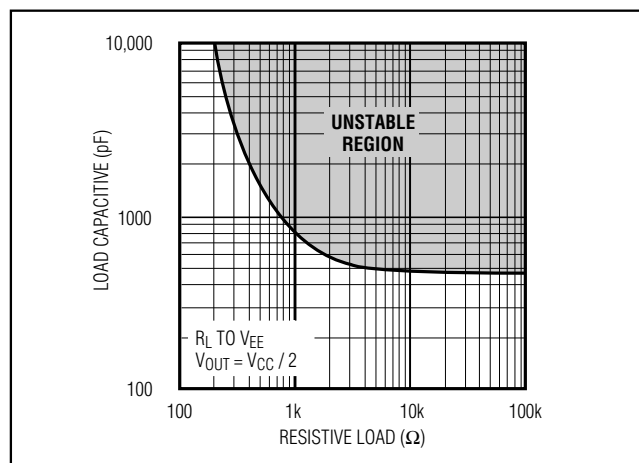
Figure 4. Capacitive-Load Stability
