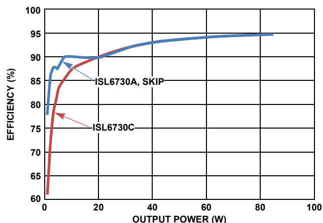
FIGURE 2. PFC EFFICIENCY
