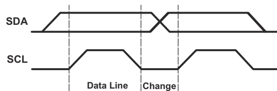
Figure 8-5. Bit Transfer
