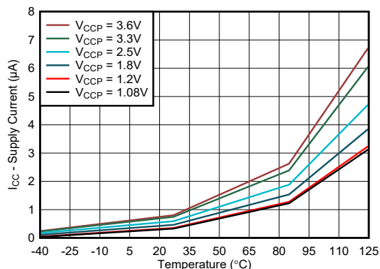
Figure 6-3. Standby Supply Current vs Temperature
