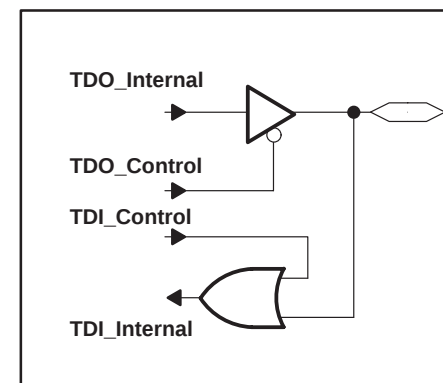
MSP430C32x: TDO/TDI MSP430P/E325A: TDO/TDI
