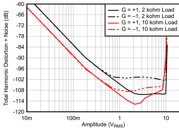
Figure 6-25. Total Harmonic Distortion + Noise Ratio vs Output Amplitude
