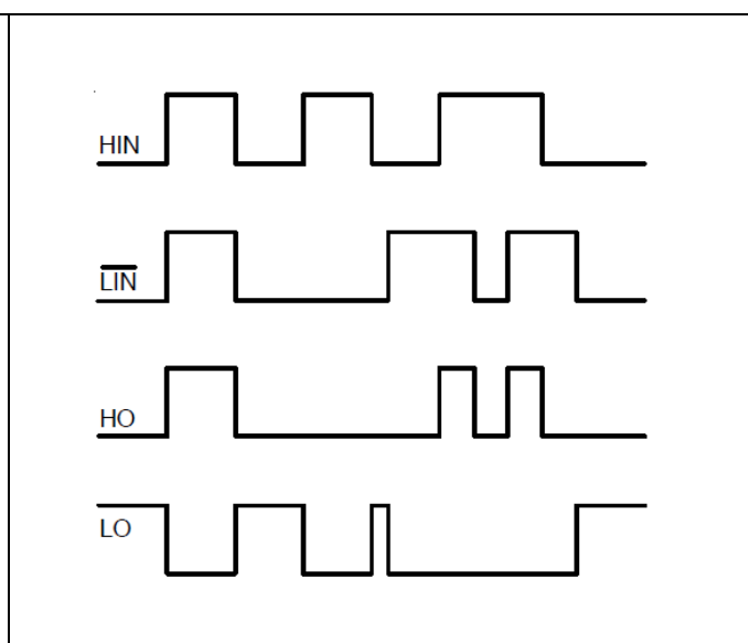
Figure 7 Input/output logic diagram
