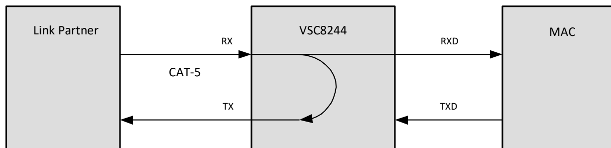
Figure 21. Far-end Loopback Block Diagram
