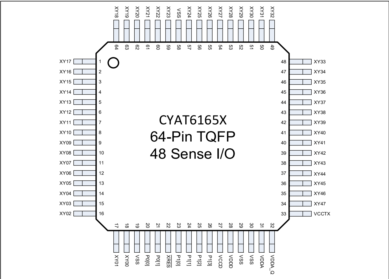
Figure 13 64-pin TQFP pinout
