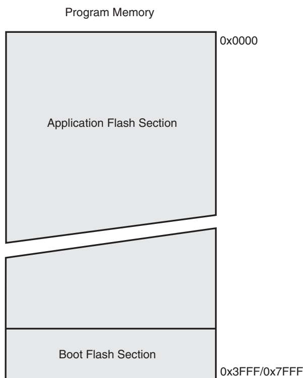
Figure 8-1. Program Memory Map
