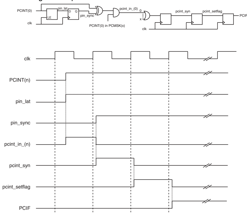
Figure 13-1. Pin Change Interrupt
