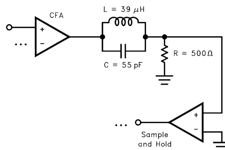
FIGURE 6. COLORBURST TRAP FOR NTSC APPLICATIONS
