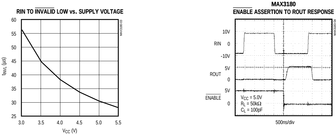
Typical Operating Characteristics (continued) (V CC = +5V, T A = +25°C, unless otherwise noted.)
