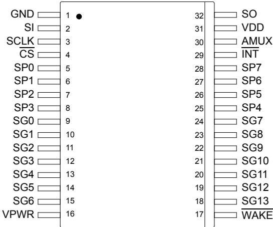
Figure 3. 33993 Pin Connections
