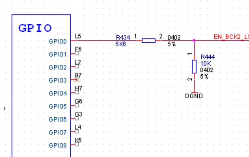
Fig. 7: Simplified schematics of EN_BCK2_LS internal pin configuration
