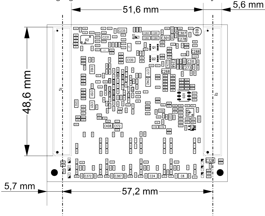
Fig. 6: Connectors layout
