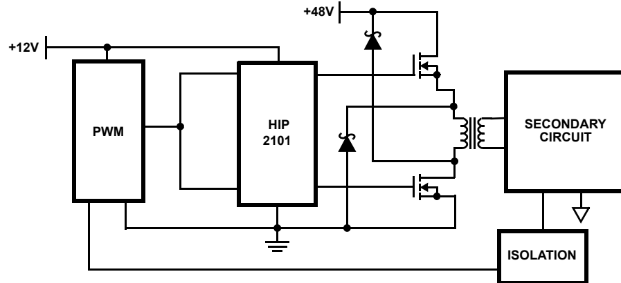
FIGURE 1. TWO-SWITCH FORWARD CONVERTER
