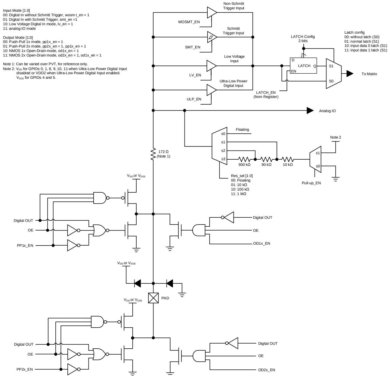
Figure 14: SLG46881 GPIO with Matrix OE and Input LATCH IO Structure Diagram
