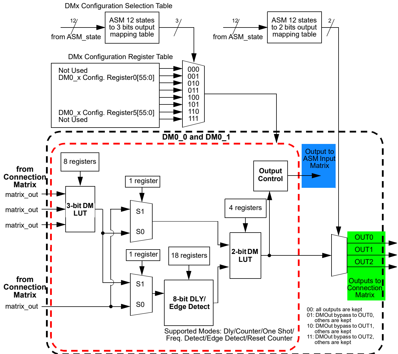
Figure 123: DM0_0/DM0_1 Outputs
