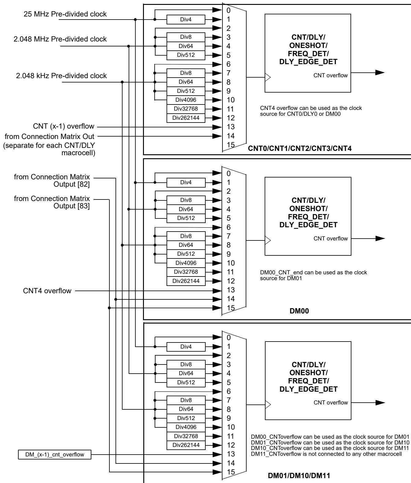
Figure 82: Clock Scheme
