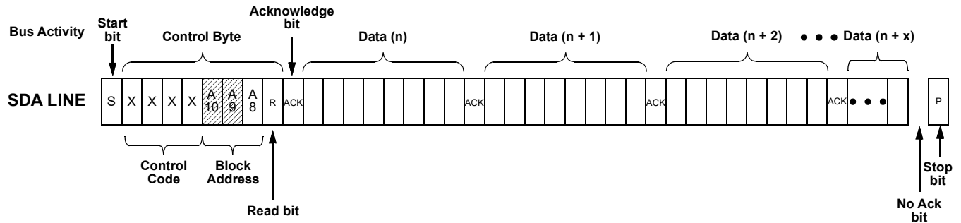
Figure 139: Sequential Read Command
