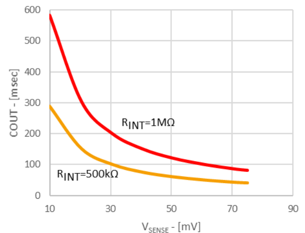
COU T Period vs V SENSE
