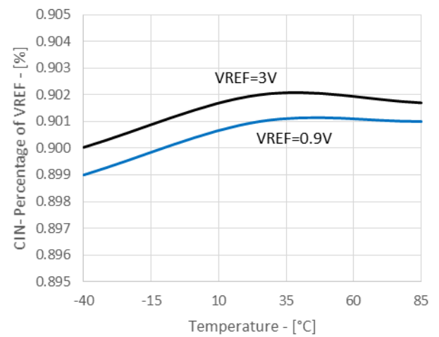
CIN- Variation Over Temperature
