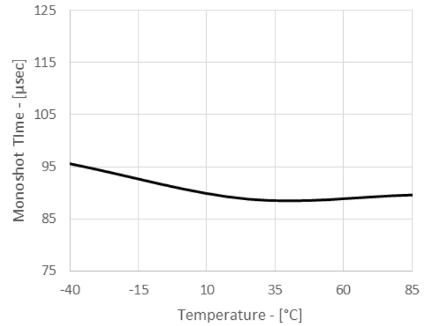
Monoshot Time vs Temperature
