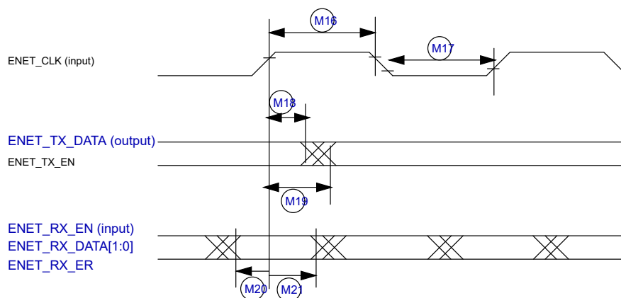
Figure 51. RMII mode signal timing diagram
