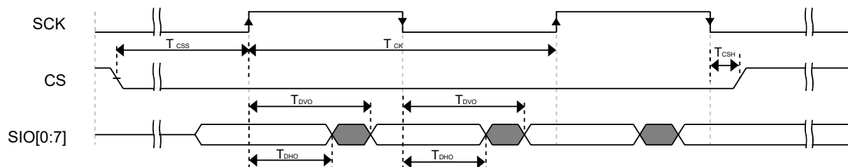
Figure 26. FlexSPI output timing in DDR mode
