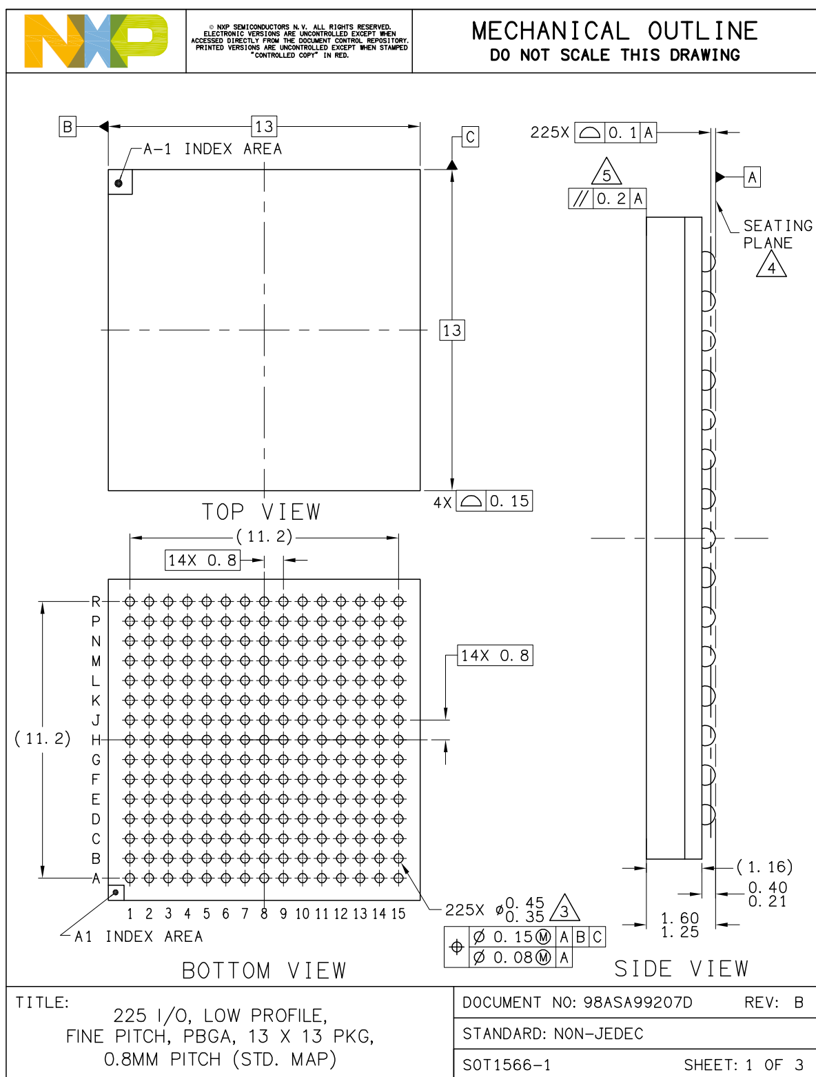
Figure 53. 13 x 13 mm BGA, case x package top, bottom, and side Views
