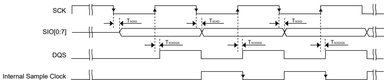
Figure 21. FlexSPI input timing in SDR mode where FlexSPIn_MCR0[RXCLKSRC] = 0X3 (case A2)
