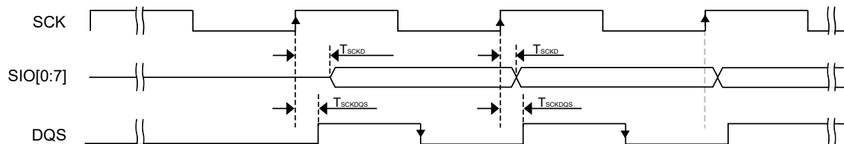
Figure 20. FlexSPI input timing in SDR mode where FlexSPIn_MCR0[RXCLKSRC] = 0X3 (case A1)
