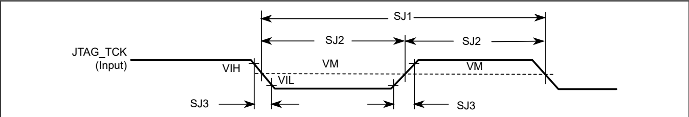
Figure 9. Test clock input timing diagram
