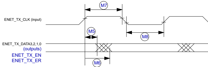
Figure 48. MII transmit signal timing diagram
