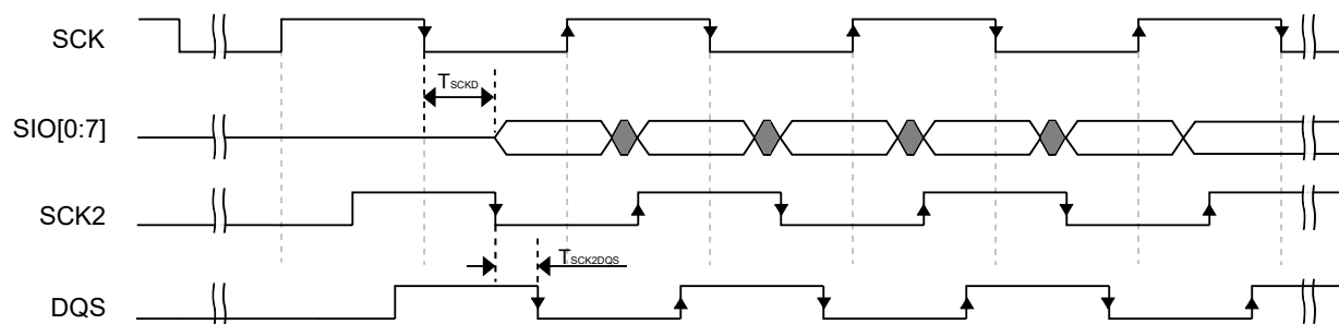
Figure 24. FlexSPI input timing in DDR mode where FlexSPIn_MCR0[RXCLKSRC] = 0x3 (case B2)
