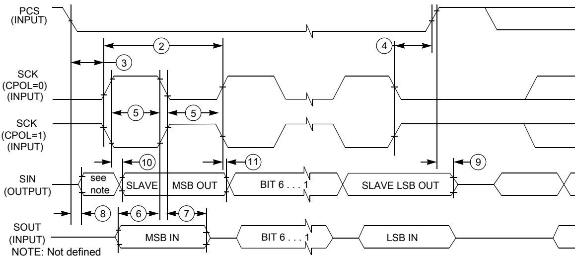
Figure 42. LPSPi Slave mode timing (CPHA = 1)
