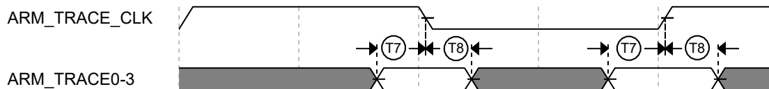
Figure 14. Trace data specifications
