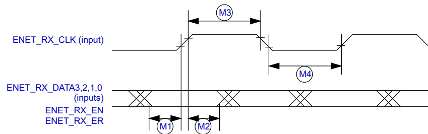
Figure 47. MII receive signal timing diagram
