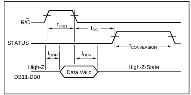
FIGURE 4. \overline{R}/\overline{C} Pulse High — Outputs Enabled Only While \overline{R}/\overline{C} Is High.
