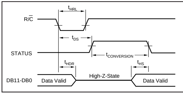
FIGURE 3. \overline{R}/\overline{C} Pulse Low—Outputs Enabled After Conversion.
