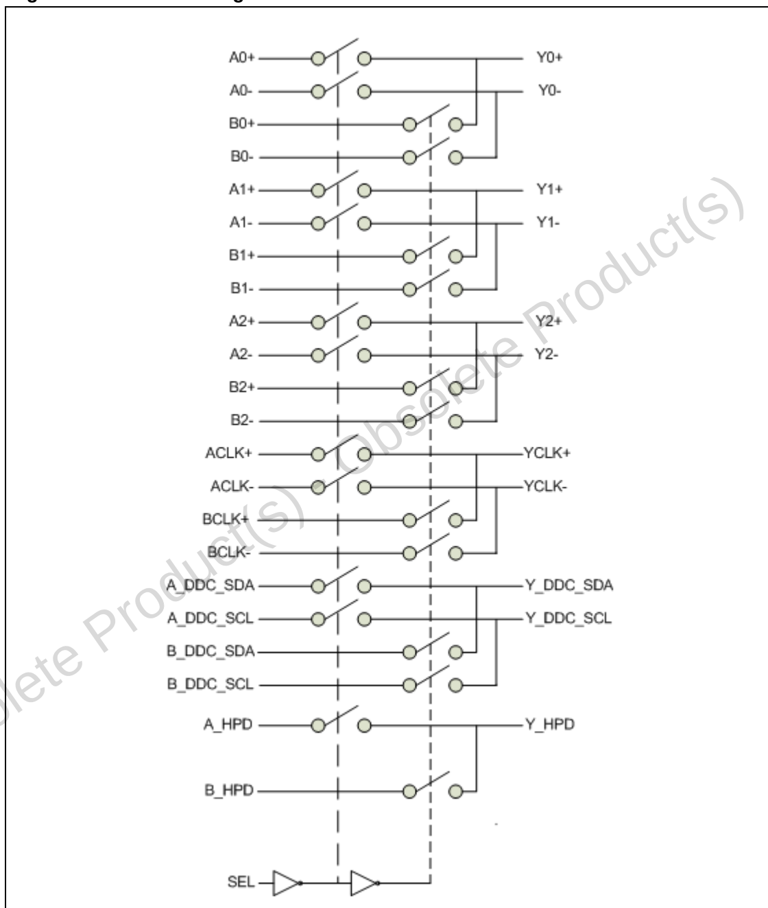
Figure 1. Functional diagram
