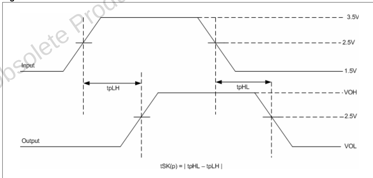
Figure 11. Pulse skew
