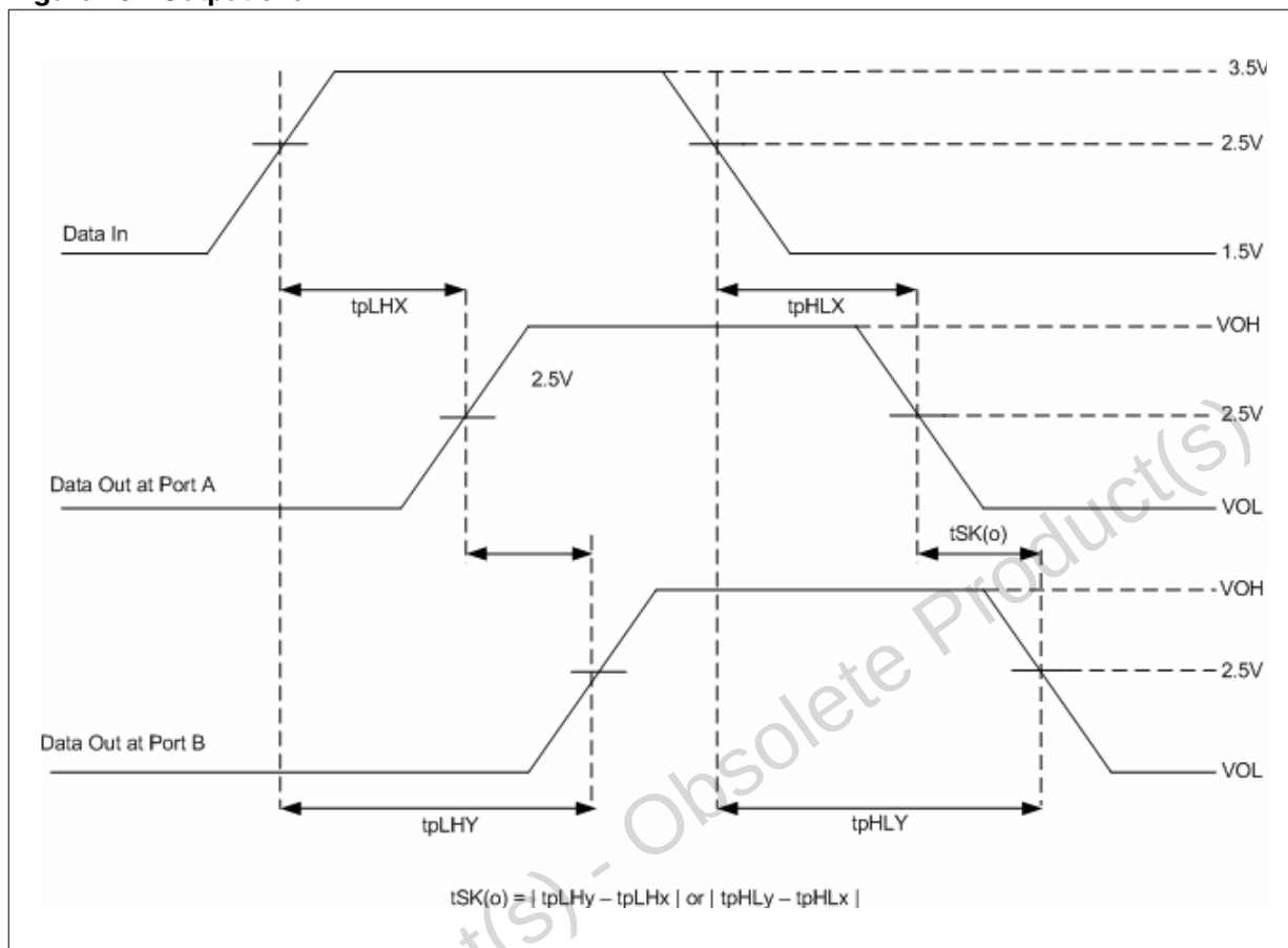
Figure 10. Output skew
