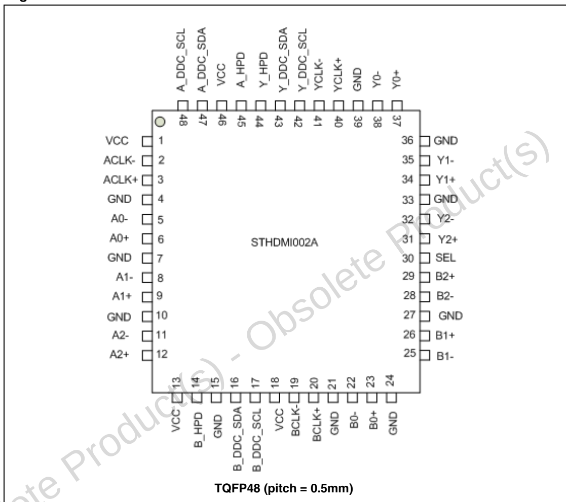
Figure 3. Pin connections
