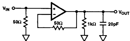
FIGURE 1. LARGE SIGNAL RESPONSE TEST CIRCUIT
