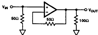
FIGURE 2. SMALL SIGNAL RESPONSE TEST CIRCUIT
