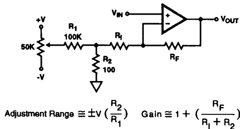
FIGURE 29. NON-INVERTING GAIN
