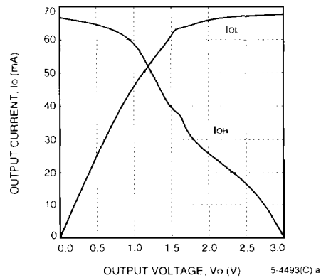
Figure 89. Fast ( T_J = 125^\circ\text{C} , V_{DD} = 3.0\text{ V} )
