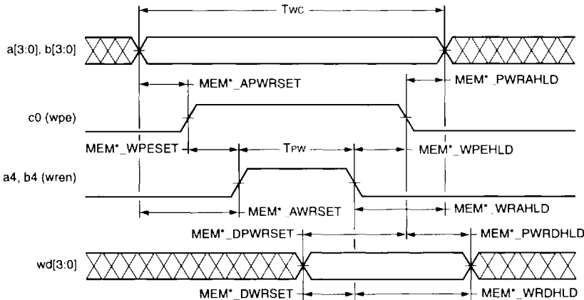
Figure 58. Write Operation
