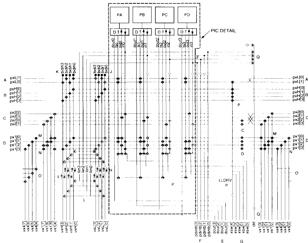
Figure 26. PIC Architecture
