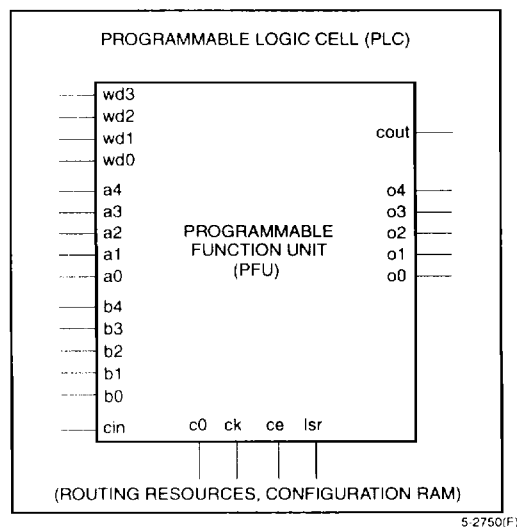
Figure 2. PFU Ports
