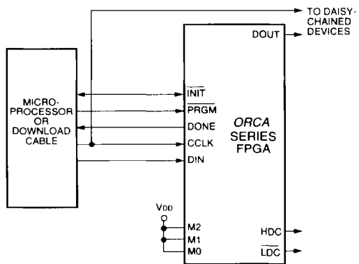
Figure 45. Slave Serial Configuration Schematic
