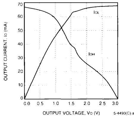
Figure 88. Slewlim ( T_J = 125^\circ\text{C} , V_{DD} = 3.0\text{ V} )
