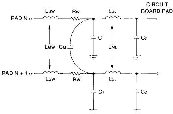
Figure 54. Package Parasitics
