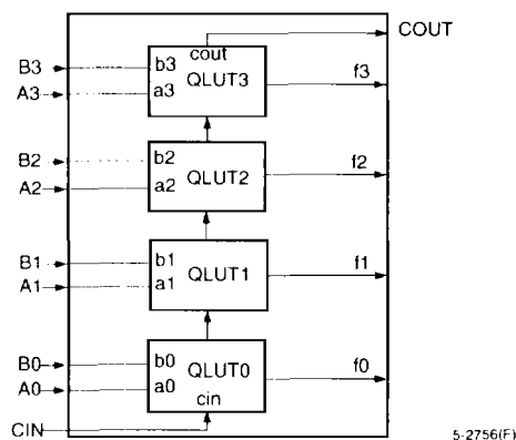
Figure 9. Ripple Mode
