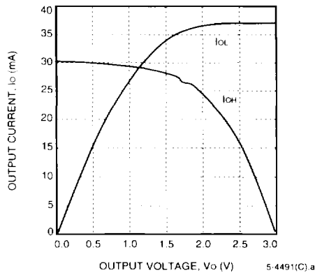
Figure 87. Sinklim ( T_J = 125^\circ\text{C} , V_{DD} = 3.0\text{ V} )
