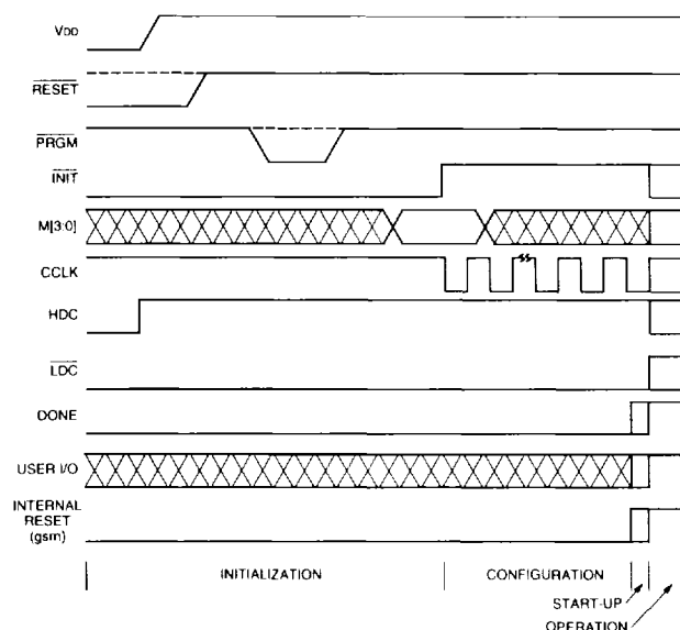
Figure 37. Initialization/Configuration/Start-Up Waveforms
