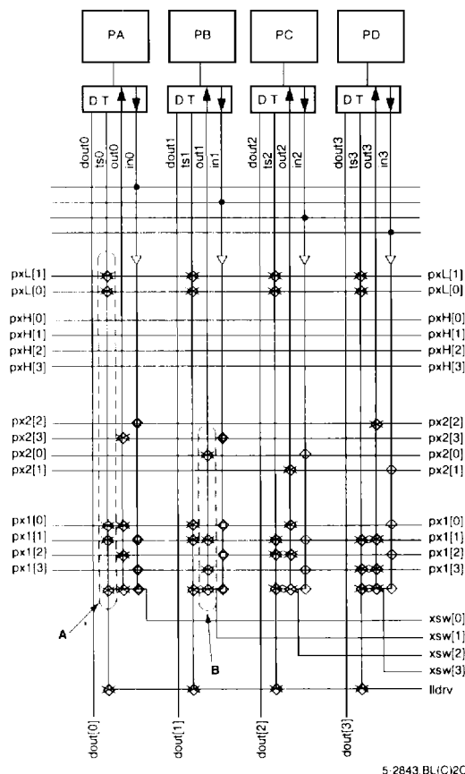
Figure 27. PIC Detail
