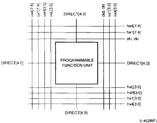
Figure 21. Single PLC View of Inter-PLC R-Nodes
