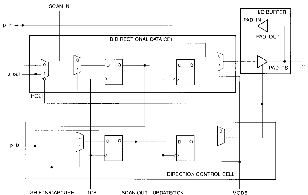
Figure 52. Boundary-Scan Cell
