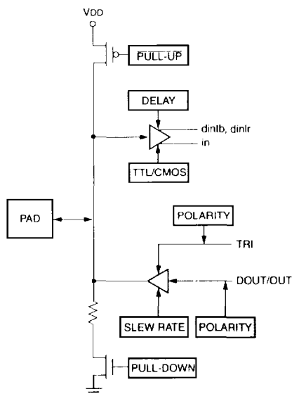
Figure 24A. Simplified Diagram of OR2CxxA Programmable I/O Cell
