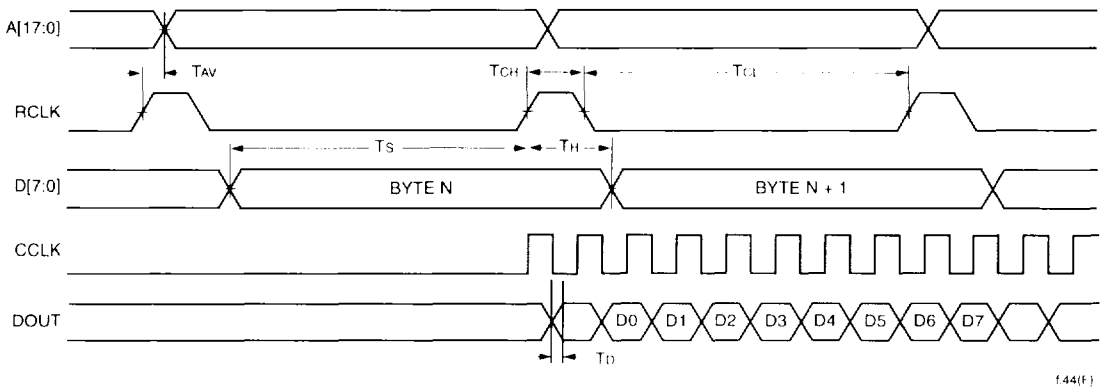
Figure 68. Master Parallel Configuration Mode Timing Diagram
