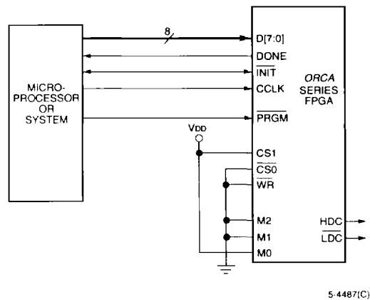
Figure 46. Slave Parallel Configuration Schematic
