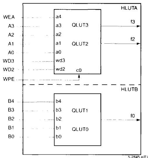
Figure 13. MA/F5 Mode— 16 \times 2 Memory and One Function of Five Input Variables
