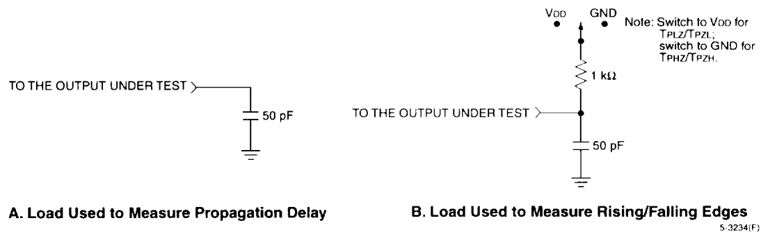
Figure 75. ac Test Loads
