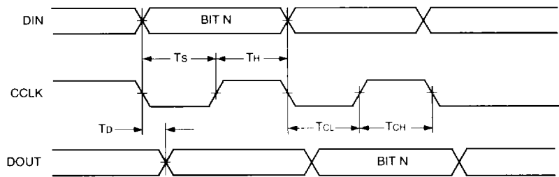
Figure 71. Slave Serial Configuration Mode Timing Diagram
