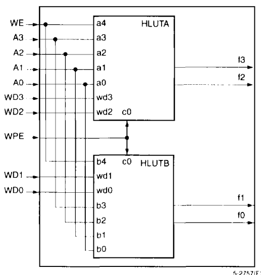
Figure 12. MA/MB Mode— 16 \times 4 RAM
